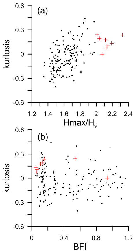
Figure 5. Plot of (a) kurtosis of the sea surface with abnormality index ( H_{max}/H_s ) and (b) kurtosis of the sea surface elevation with Benjamin–Feir index (BFI). The data of the freak waves are indicated with cross symbols.
