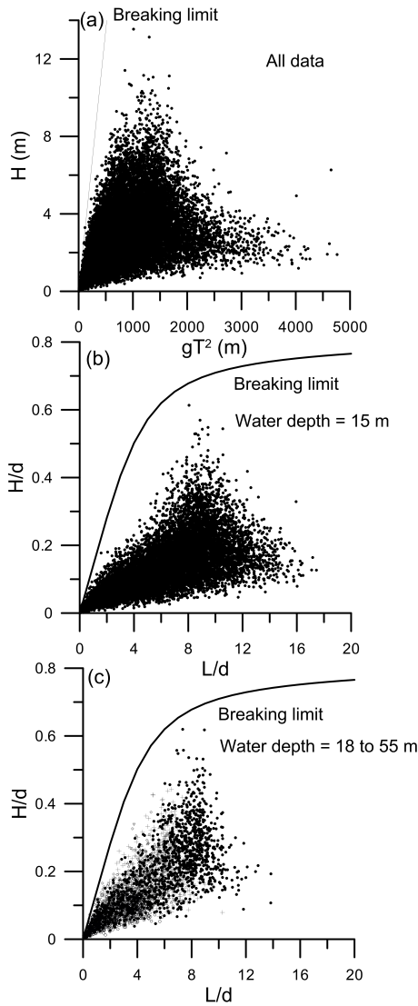
Figure 11. The graph showing the breaking limit based on (a) Ochi (1990) for all data, (b) Fenton (1990) for data at 15 m water depth and (c) Fenton (1990) for data at 18 to 55 m water depth.
