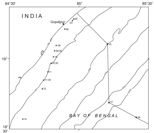
Figure 2. Cyclone track (solid circle) connected with straight line and Waverider buoy location (star) at different time on 12 October 2013. The time in UTC is indicated near the points.
