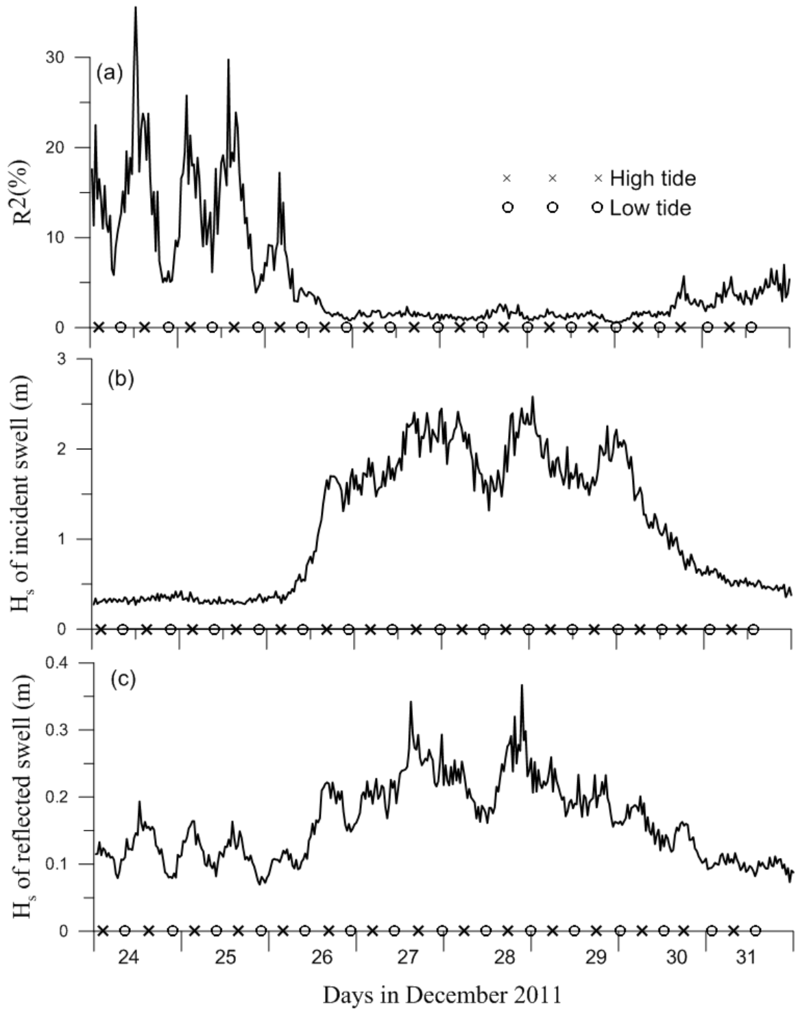
Figure 7. Wave reflection parameters off Visakhapatnam coast during severe cyclonic storm THANE (a) percentage of reflection (b) H_s of incident swell and (c) H_s of reflected swell
