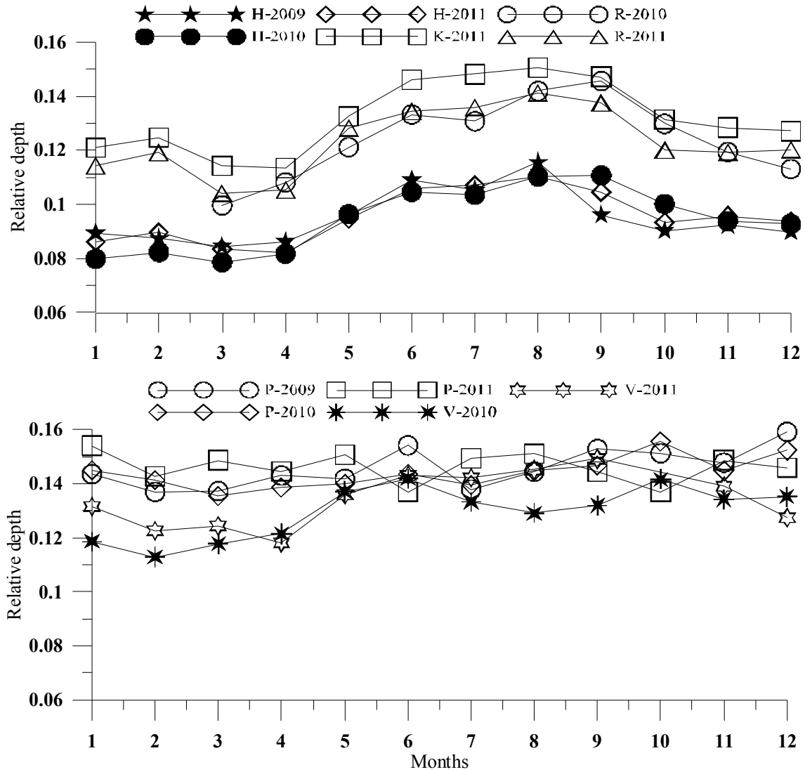
Figure 3. Monthly average of relative depth for locations along west coast (top panel) and that along east coast (bottom panel) of India in different months
