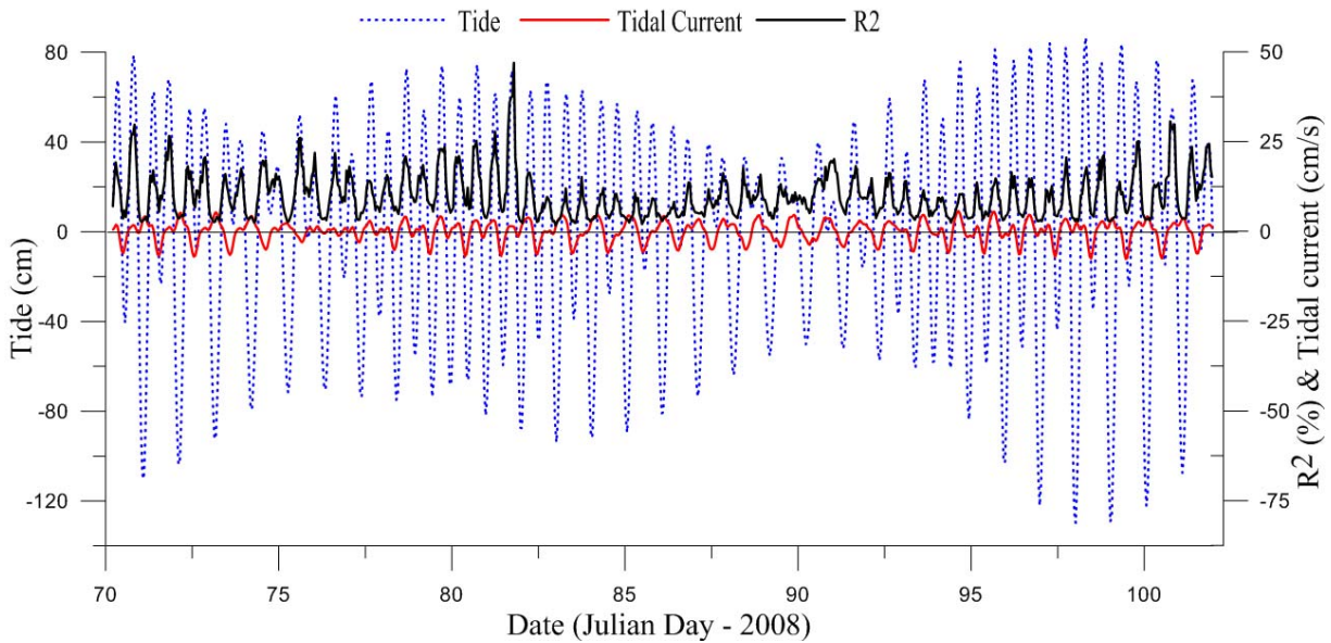
Figure 8. Effect of tide and tidal current on wave reflection coefficient off Honnavar
