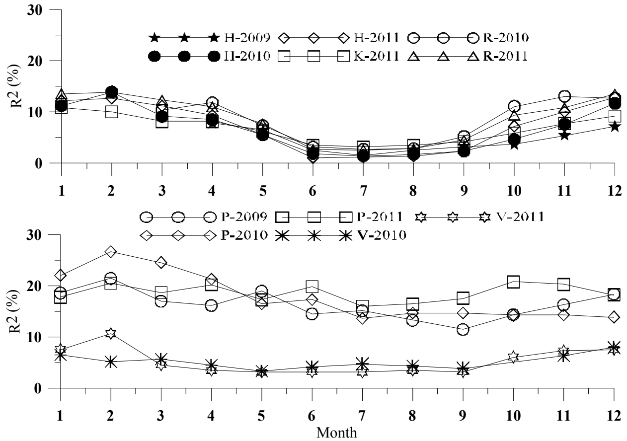
Figure 2. Monthly average percentage of reflected incident energy off west coast (top panel) and east coast of India (bottom panel) in different months
