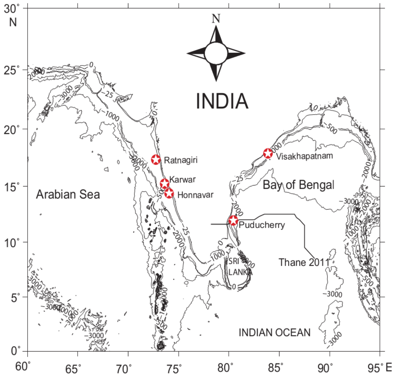
Figure 1. Study area and track of severe cyclonic storm 'THANE'. The depth contours are in meters
