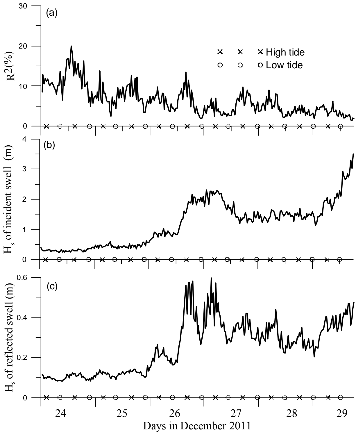
Figure 6. Wave reflection parameters off Puducherry coast during severe cyclonic storm THANE (a) percentage of reflection (b) H_s of incident swell and (c) H_s of reflected swell
