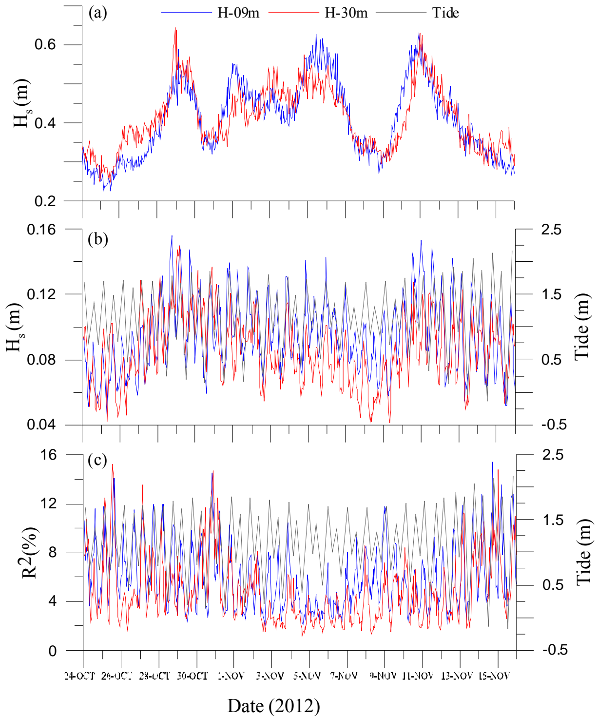
Figure 5. Hourly averaged (a) Incident wave height (b) reflected wave height and (c) reflection coefficient off Honnavar at 9 m and 30 m water depth
