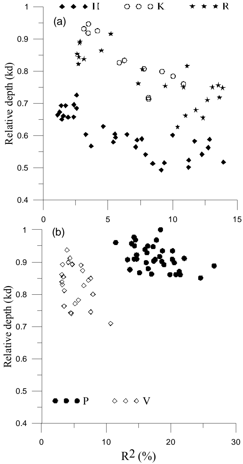
Figure 4. The plot of percentage of reflection with relative depth (a) for locations along the west coast and (b) for locations along the east coast of India
