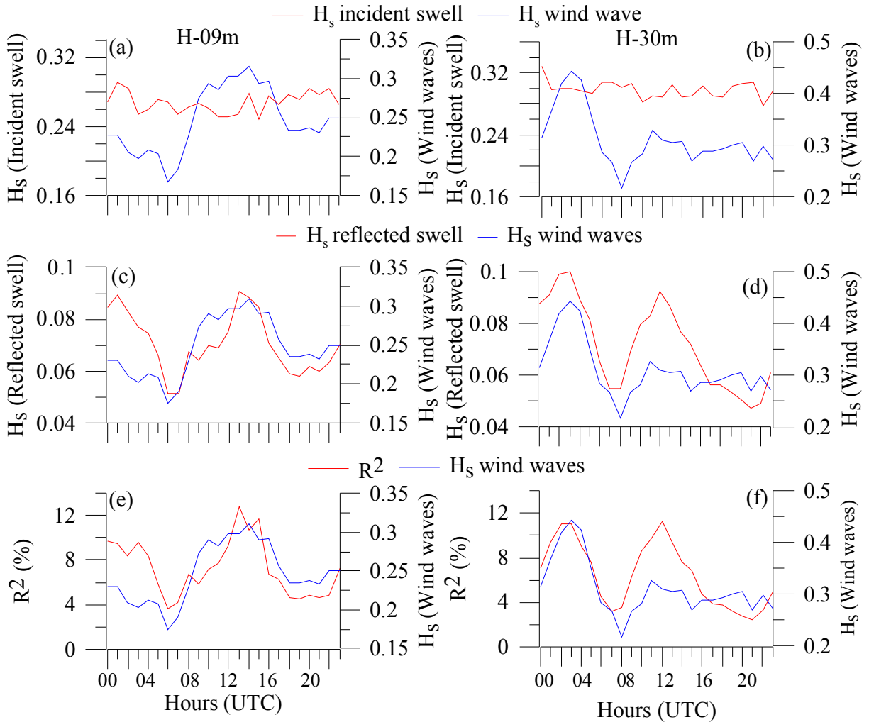
Figure 9. Effect of land/sea breeze on (a,b) incident swell (c,d) reflected swell (e,f) R^2 off Honnavar at 9-m and 30-m water depth
