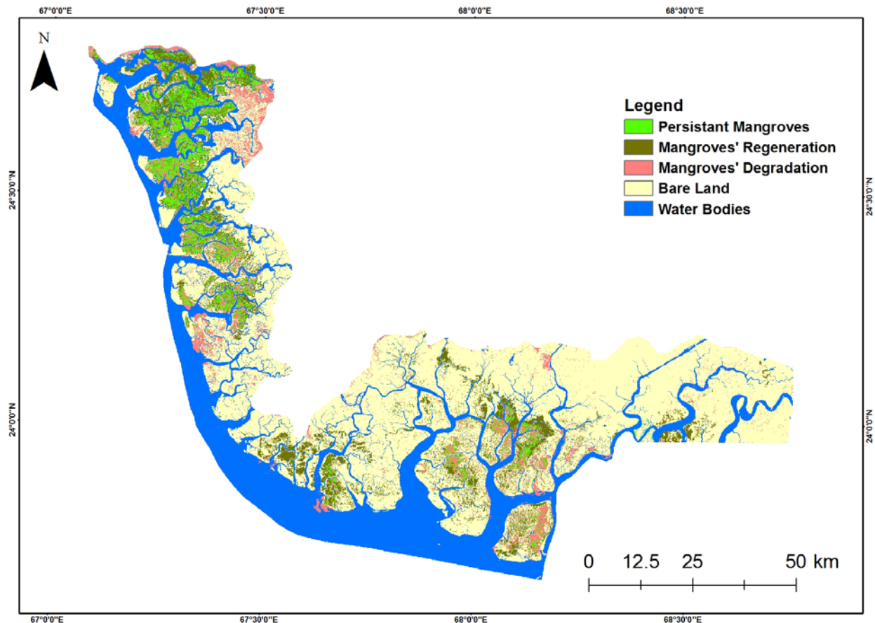
Figure 2: Persistent mangroves with forest loss and gain of Indus Delta from 1973 to 2010.
