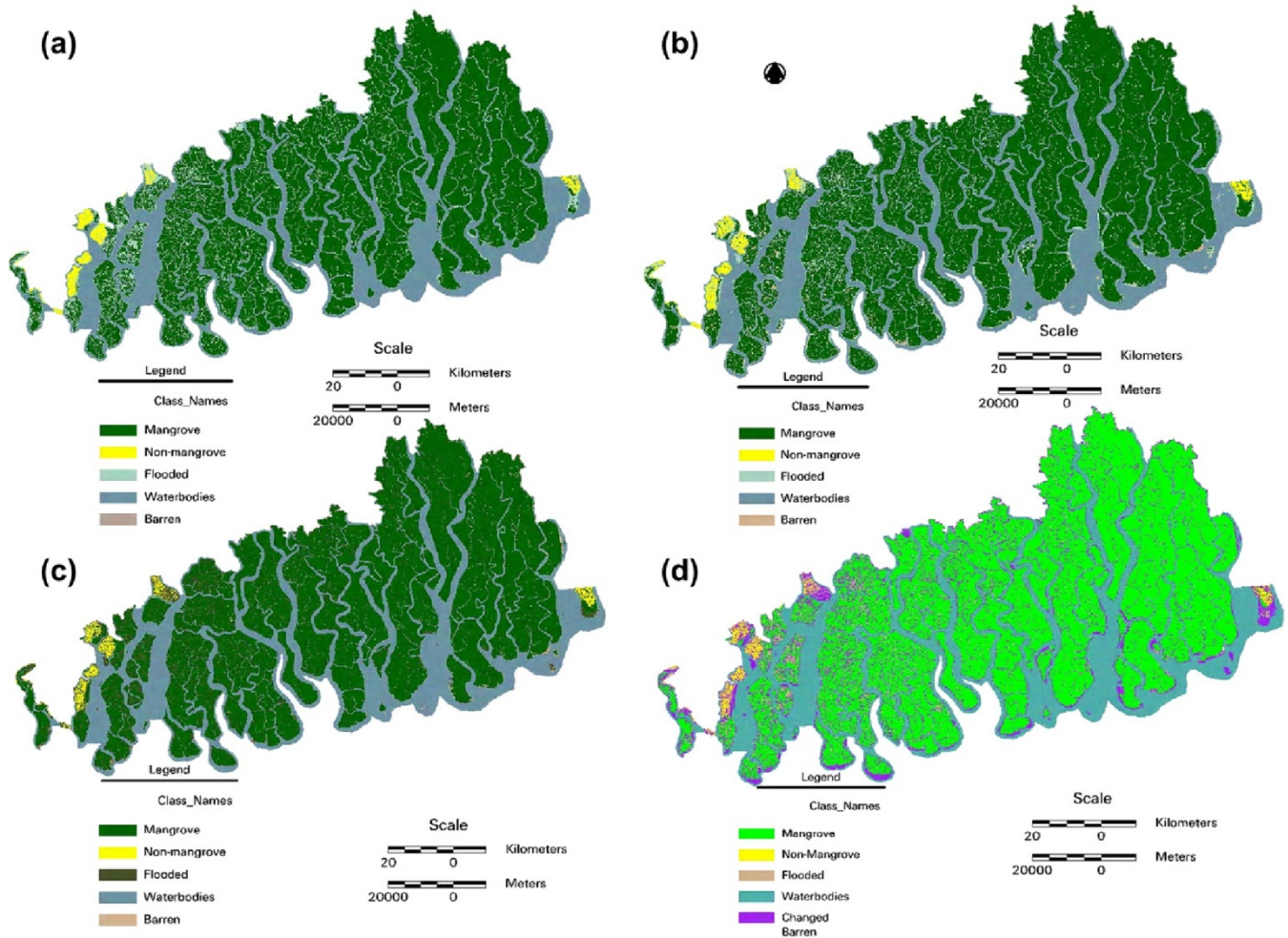
Fig. 4 Classification maps of (a) MSS, (b) TM, and (c) ETM + data, and (d) change maps from the 1970s to 2000s
