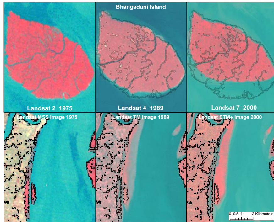
Figure 5: Example of erosion and aggradation in Sundarban (red color represents mangroves)
