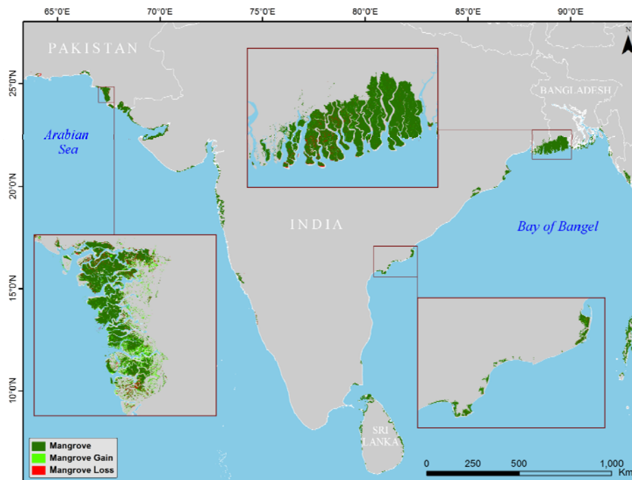
Figure 1: Persistent mangroves of South Asia with forest gain and loss from 2000 to 2012
