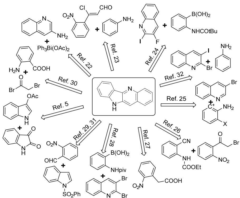
Figure 2. Synthetic approaches to 10 H -indolo[3,2- b ]quinoline.
