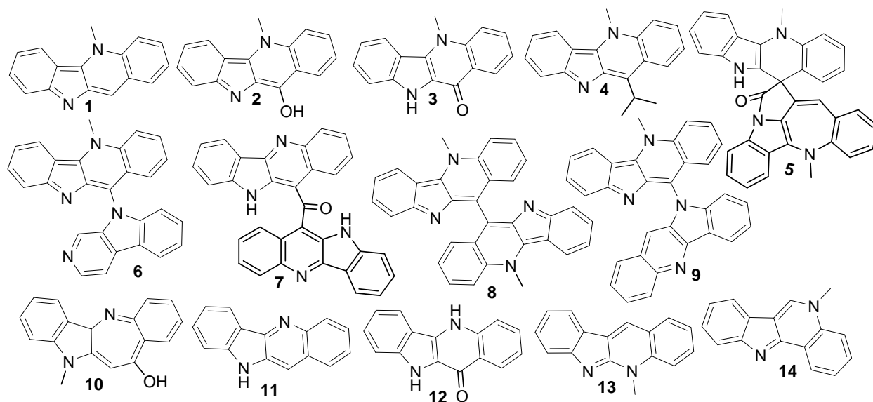
Figure 1. Structures of indoloquinoline alkaloids isolated from Cryptolepis sanguinolenta .
