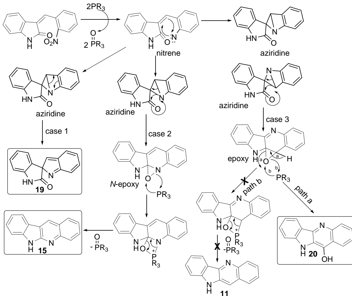
Scheme 3. Proposed mechanism for the formation of indoloquinolines and spiro[2 H -indole-2,3'-oxindole]
