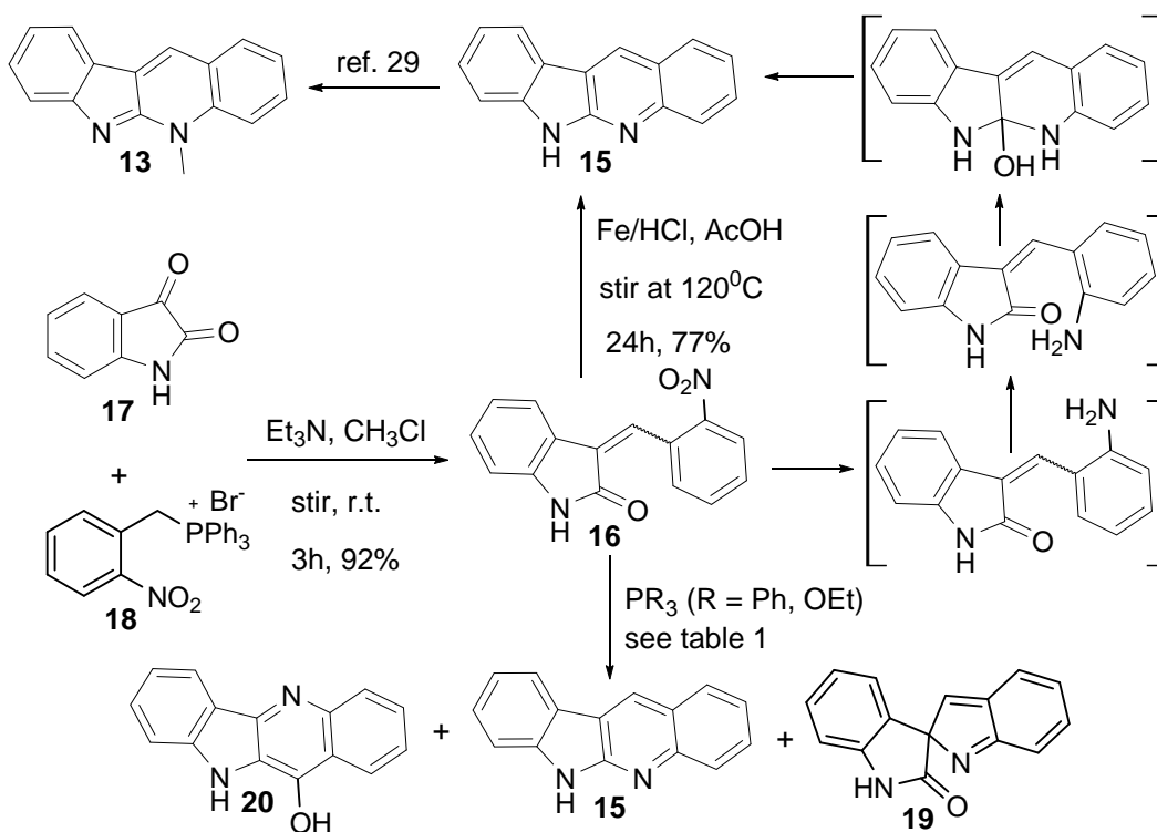
Scheme 2. Synthesis of indoloquinolines and spiro[2H-indole-2,3'-oxindole]
