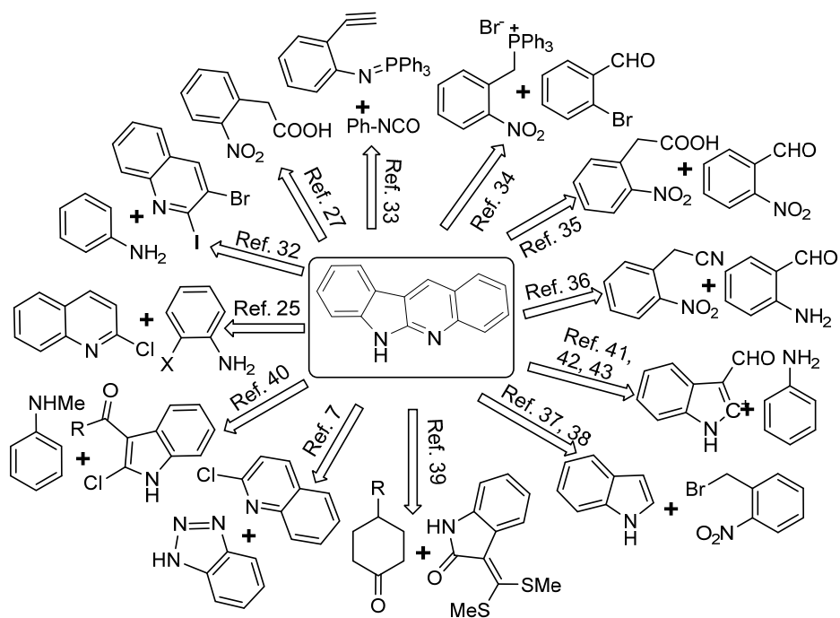
Figure 3. Synthetic approaches to 6 H -indolo[2,3- b ]quinoline.
