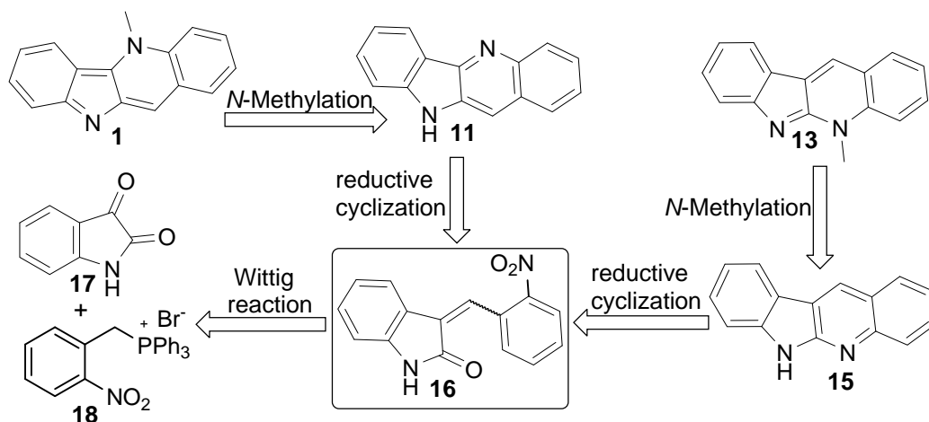
Scheme 1. Retrosynthetic analysis of cryptolepine and neocryptolepine
