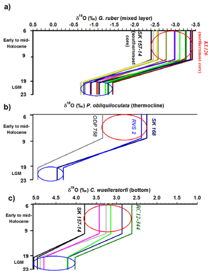
Fig. 8. Schematic representation of the LGM to mid-Holocene differences in \delta^{18}\text{O} surface, thermocline and bottom waters in the N-S transect a) Surface water \delta^{18}\text{O} ( G. ruber ; 20° N to 5°N); b) Thermocline \delta^{18}\text{O} ( P. obliquiloculata for core SK 168 and RVS 2 and N. dutertrei for core ODP 758 (12°N to 5°N); c) Bottom water \delta^{18}\text{O} ( C. wuellerstorfi (13°N to 5°N).
