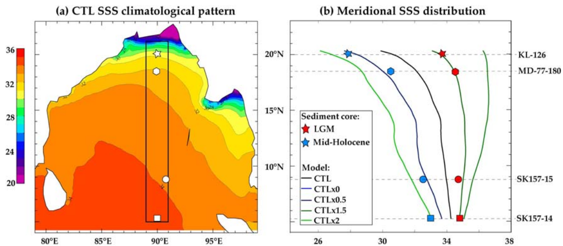
Fig. 10. Model freshwater sensitivity experiments a) CTL sea surface salinity with 90°E meridional transect outlined; b) Meridional sea surface salinity transects averaged between 89°E and 91°E (black frame on panel a) for CTL and sensitivity experiments where a constant coefficient \alpha is applied to the total fresh water forcing ( \alpha ; CTLx0, CTLx0.5, CTLx1.5 and CTLx2). Proxy sea surface salinity estimates from sediment cores in the northern and southern BoB (indicated by symbols on panels a) are also reported for mid-Holocene and LGM climate on panel b.
