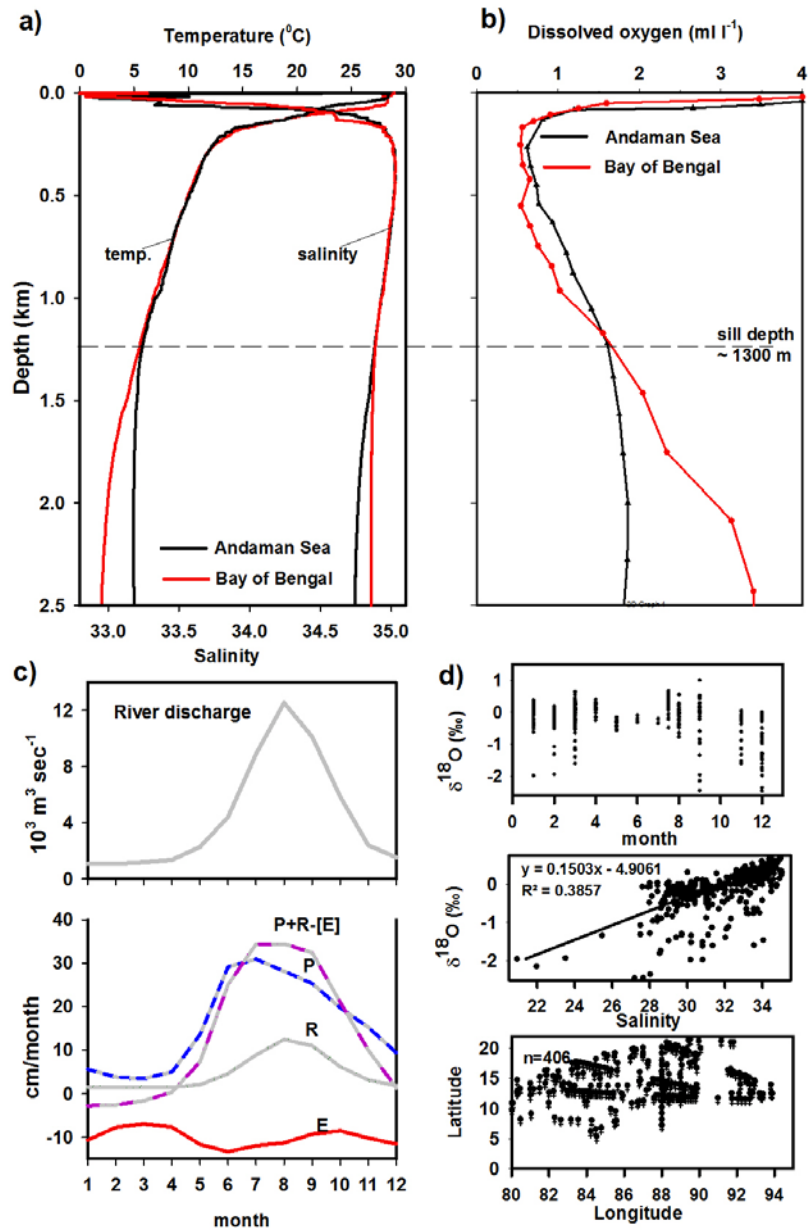
Fig. 2. a) Vertical profiles of temperature and salinity at two representative CTD stations in the Andaman Sea (10.25 N/94.078 E) and the Bay of Bengal (12.15 N/ 91.415 E); b) dissolved oxygen data from the BoB and the Andaman Sea (Naqvi et al., 1994); c) Average annual cycle of river discharge from the major rivers (Ayeyarwady, Ganges, Brahmaputra, Mahanadi, Godavari, Krishna and Cauvery) (Data source: http://www.sage.wisc.edu/riverdata/ ) and annual cycle of evaporation (E), river discharge (R), precipitation (P), P+R-(E) in the BoB (Rao and Sivakumar, 2003); d) δ 18 O sea water data versus month, surface δ 18 O-salinity relationship for the BoB (Achyuthan et al., 2013; Schmidt et al., 1999; Sengupta et al., 2013) and spatial distribution of sampling sites in the BoB (latitude versus longitude).
