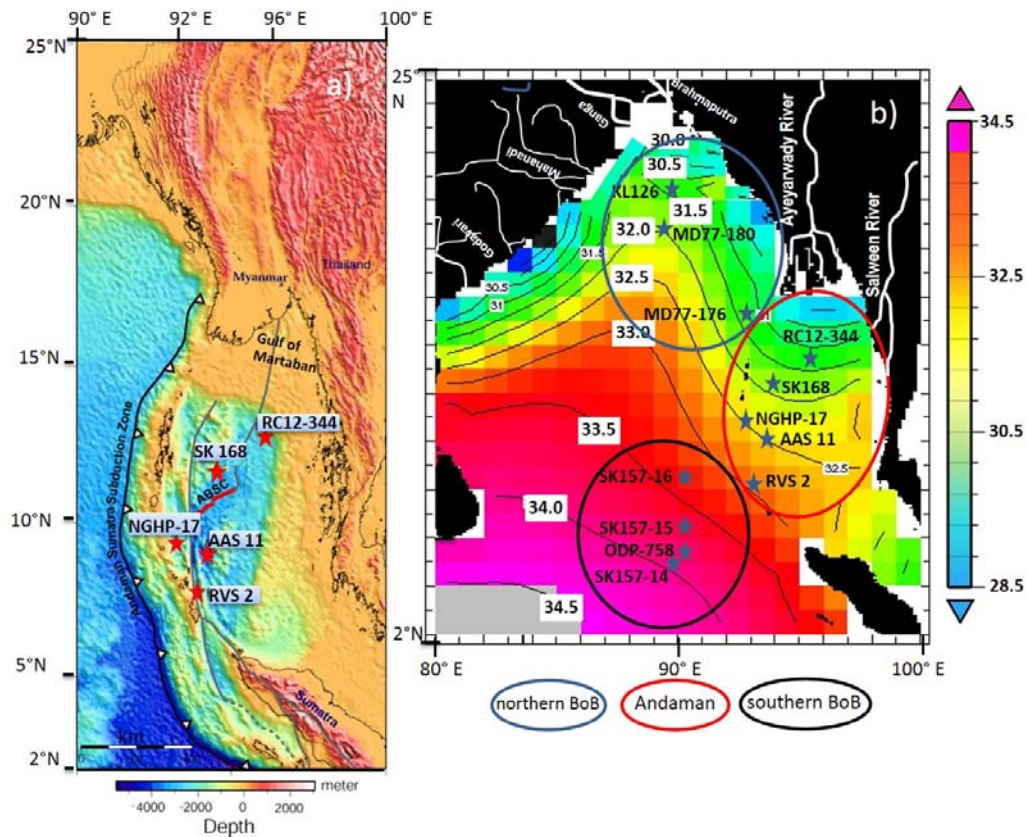
Fig. 1. Location map a) bathymetry of core locations in the Andaman Sea; b) Location of the sediment cores used in the BoB. Color shading is the present day annual average surface salinity (data from Levitus et al. (1994))
