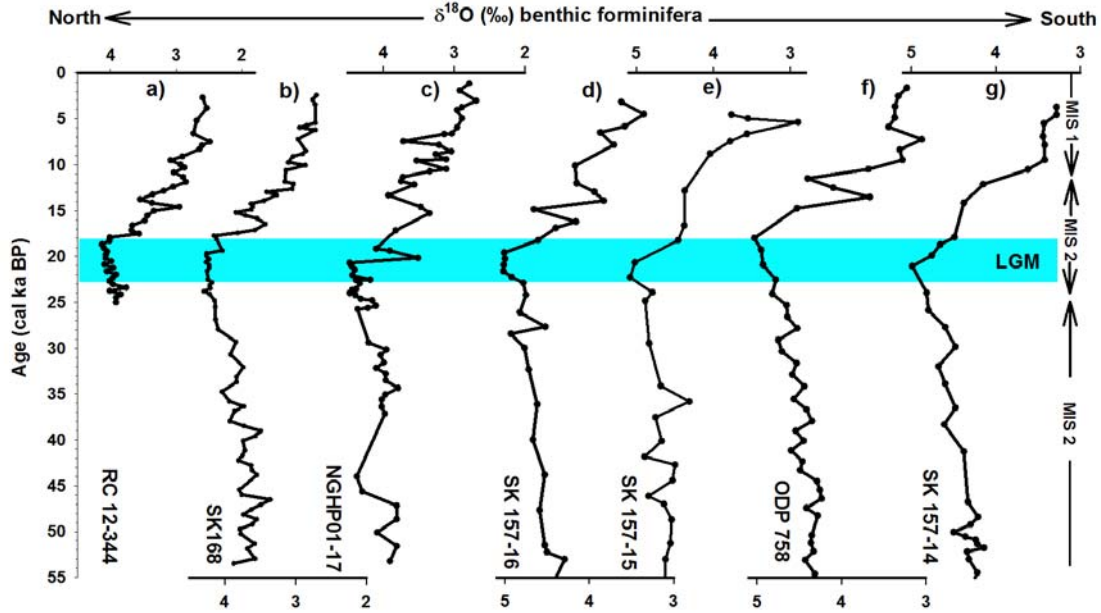
Fig. 7. Benthic oxygen isotope records. a) RC 12-344 (Naqvi et al., 1994); b) core SK 168; c) NGHP-17 (Ali et al., 2014); d) SK157-16 (Raza et al., 2014); e) SK 157-15 (Raza et al., 2014); f) ODP 758 (Bolton et al., 2013); g) SK 157-14 (Ahmad et al., 2008).
