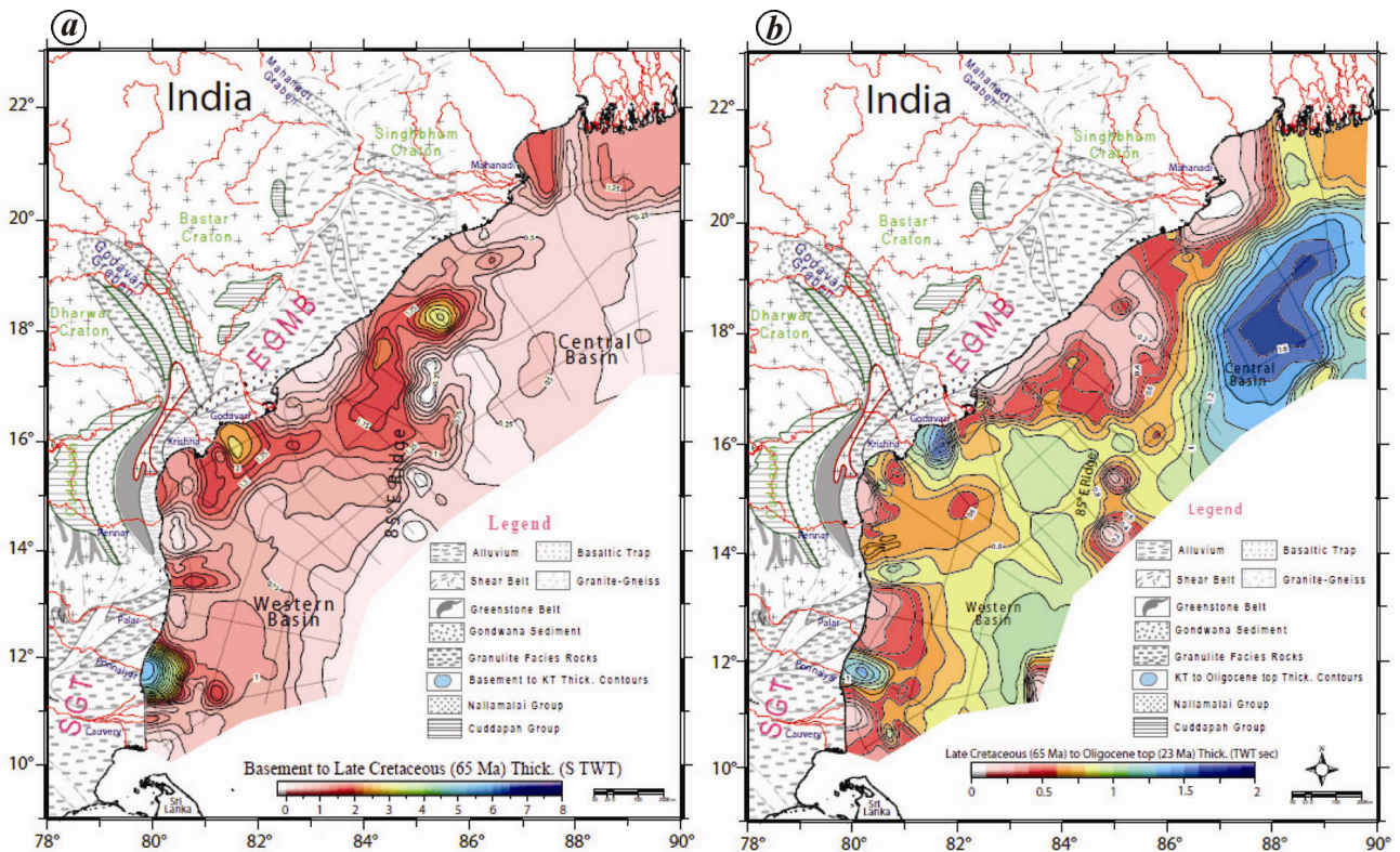
Figure 7. Sediment isopach maps prepared from the interpreted seismic reflection results. a. From basement to 65 Ma seismic horizon (contour interval 0.25 sec). b. For sediment layer deposited between 65 and 23 Ma (contour interval 0.1 sec).
