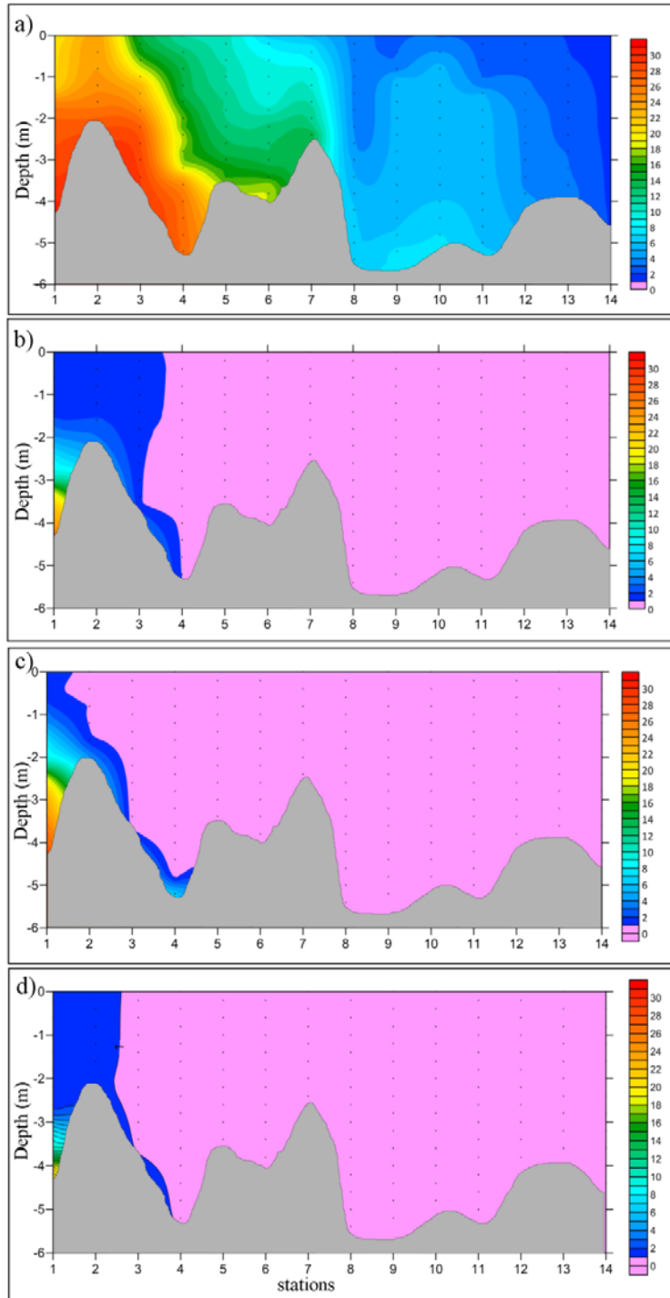
Figure 2 - Vertical distribution of salinity during (a) Pre-Monsoon, (b) Onset/first sampling of the Southwest Monsoon (Monsoon 1), (c) second sampling during the Southwest Monsoon (Monsoon 2) and (d) third sampling during the Southwest Monsoon (Monsoon 3). Salinity gradients along the study area was prominent during the Pre-Monsoon with polyhaline salinity in the downstream and oligohaline salinity in the upstream locations. During the onset of southwest monsoon, freshwater dominated the entire study area with oligohaline salinity in the downstream and limnohaline salinity in the upstream locations. During the Southwest Monsoon sampling, salt water intrusions into the backwaters was restricted to the locations very close to the barmouth. Salt wedge formation is clear in the downstream locations prominently during the Pre-Monsoon.
