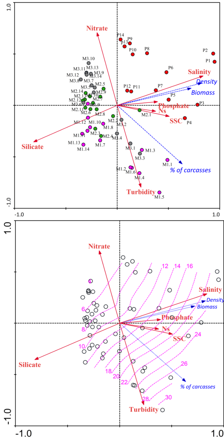
Figure 10 - RDA Triplots explains the distribution and interrelationship between the environmental and biological variables. Panel (a) represents the basic RDA plot showing the distribution of various parameters and their inter-relationships. Panel (b) represents the carcasses overlaid (contours) plot clearly evidencing the gradients in carcasses distribution and their relation with other parameters. Red dots (P1- P14) represent Pre-Monsoon, pink dots (M1.1 – M1.14) represent Monsoon 1, green dots (M2.1 – M2.14) represent Monsoon 2 and grey dots (M3.1 – M3.14) represent Monsoon 3.
