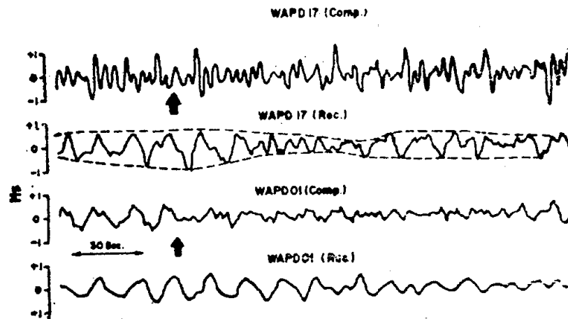
Fig. 1. Recorded (Rec) and computed (Comp) surface wave profiles for a narrow band swell (WAPD01) and a wide band multip peaked sea state (WAPD17).
