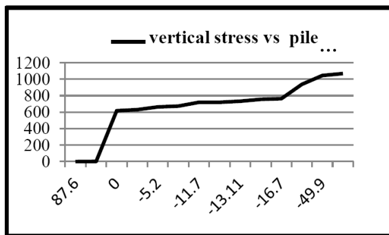
Fig 5: Vertical stress at corresponding pile depth
