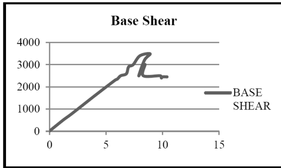
Fig 7: The base shear characteristic of static pile
