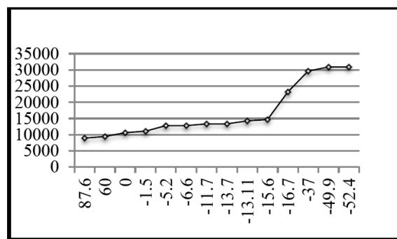
Fig 6: Cumulative Skin Friction (kN/m) Vs Depths
