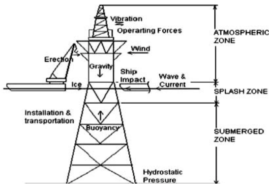
Fig 1: The loads on the structure (Chakrabarti, 2005)
