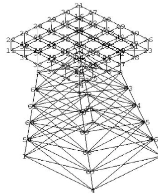
Fig 2: Joint Number Provided in STRUCAD 3D model
