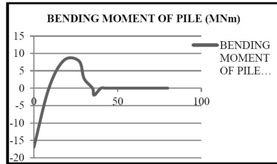
Figure 8: Bending Moment of Pile Vs Depth
