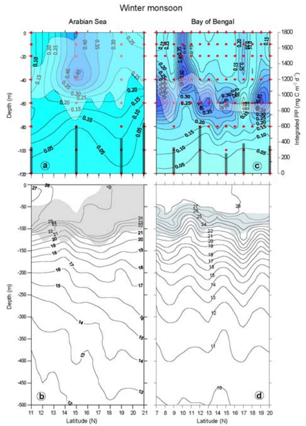
Figure 2. Vertical distribution of chlorophyll a ( \text{mg}/\text{m}^3 ) (a & c) and temperature (b & d) in the Arabian Sea (a & b) and the Bay of Bengal (c & d) during winter monsoon. The shaded region within the broken line in a & c denotes the region with nitrate concentration of 0.2 to 4 \mu\text{M} and vertical bar is the column integrated (up to 120 \text{ m} ) primary productivity ( \text{mg C m}^{-2} \text{ d}^{-1} ). The shading in b & d is the region of nitracline with nitrate concentration of 2 to 20 \mu\text{M} .
