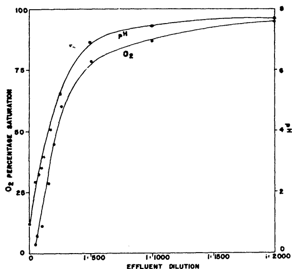
Fig. 1—Changes in pH and oxygen percentage saturation at different dilutions of the effluent
