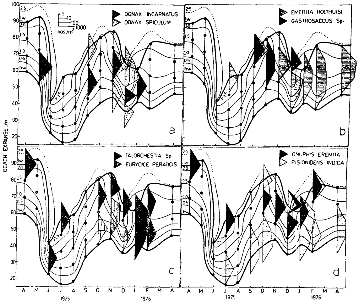
Fig. 10 (a-d) — Kite diagrams showing distribution and abundance of macrofaunal elements for different months superimposed on beach profile contours [Closed circles indicate the absence on the sampling date]
