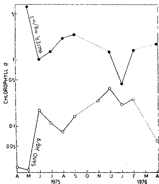
Fig. 8 — Chlorophyll a content in surf-water and in surf-sand for different months
