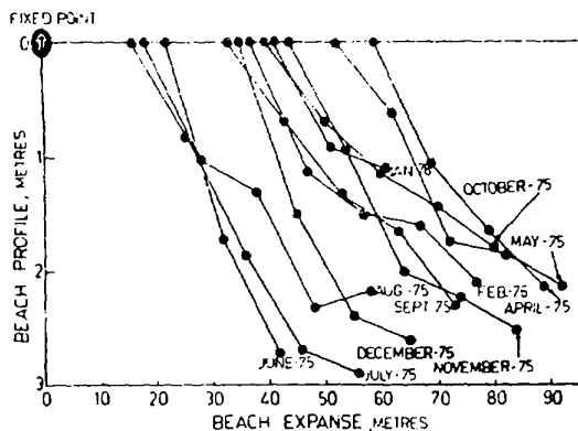
Fig. 1—Beach profiles for Baina for different months measured from a fixed point
