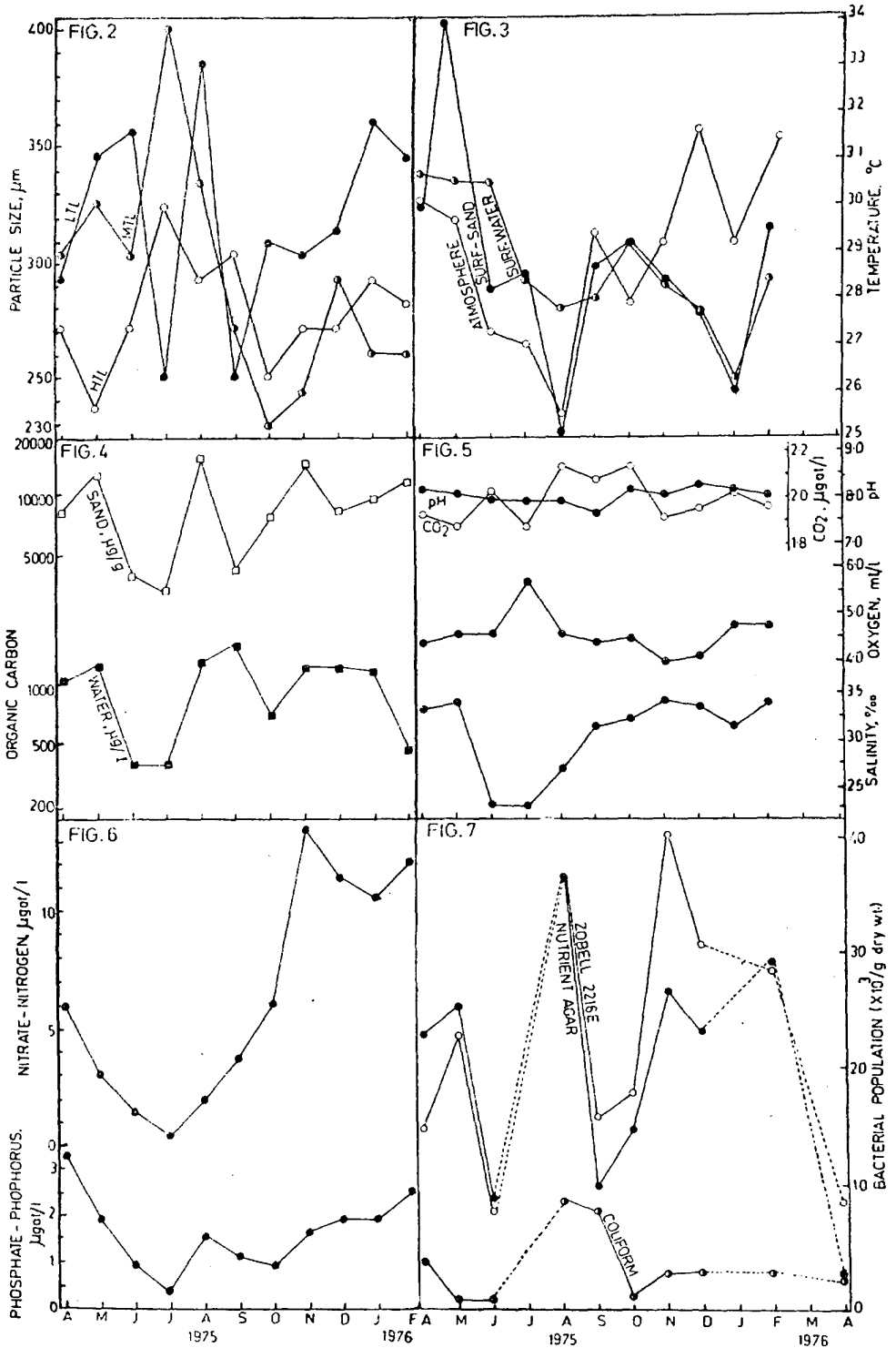
Fig. 2 — Median particle size of sand of different tide levels for different months. Fig. 3 — Temperature of atmosphere, surf-sand and surf-water for different months. Fig. 4 — Particulate organic carbon content in sand and in surf-water for different months. Fig. 5 — Salinity, dissolved oxygen, pH and \text{CO}_2 of surf-water for different months. Fig. 6 — Phosphate-phosphorus and nitrate-nitrogen content in surf-water for different months. Fig. 7 — Total bacterial population and coliform population in sand for different months
