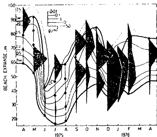
Fig. 9 — Kite diagrams showing biomass of macrofauna at different stations for different months superimposed on beach profile contours [Closed circles indicate absence on the sampling date. hw — high water mark; lw — low water mark]
