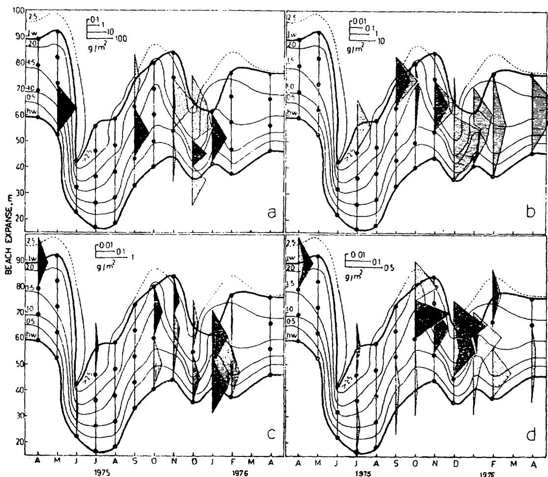
Fig. 11(a-d) — Kite diagrams showing biomass of macrofaunal elements for different months [Symbols as in Figs. 10a-d]
