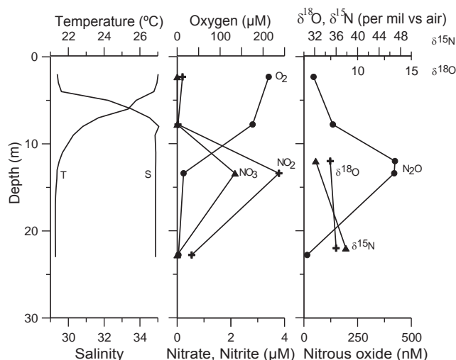
Fig. 7. Vertical profiles of temperature, salinity, dissolved \text{O}_2 , inorganic nitrogen species and \delta^{15}\text{N} and \delta^{18}\text{O} of \text{N}_2\text{O} at Sta. SK 137/39 ( 9.950^\circ\text{N} ; 76.017^\circ\text{E} ; Fig. 1) sampled on 8 August 1998. These data are hitherto unpublished.
