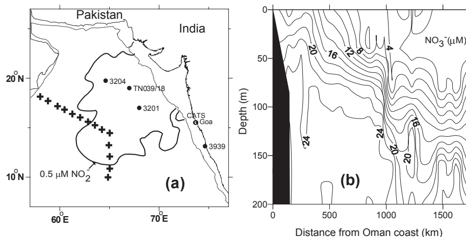
Fig. 1. (a) Geographical limits of the offshore suboxic zone as demarcated by the 0.5 \mu\text{M NO}_2^- contour (redrawn from Naqvi, 1991). Also shown are the stations (marked by crosses) worked during the U.S. JGOFS cruise TN050 (August–September 1995), whose data have been used to construct the \text{NO}_3^- section shown in (b), as well as some other stations (marked by circles) mentioned elsewhere in the paper. Isopleths in (b) and Figs. 2–4 were drawn using Surfer ® for Windows version 8 by Golden Software, Inc.
