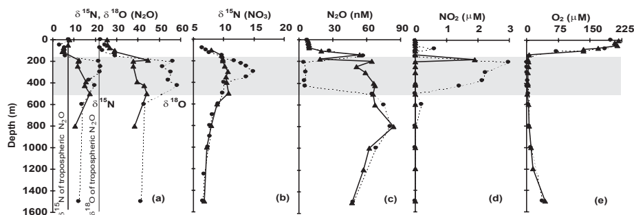
Fig. 6. Vertical profiles of \delta^{15}\text{N} and \delta^{18}\text{O} (‰ relative to air; see footnote #3) of \text{N}_2\text{O} (a), \delta^{15}\text{N} of \text{NO}_3^- (b), and concentrations of \text{N}_2\text{O} (c), \text{NO}_2^- (d) and \text{O}_2 (e) at stations SS 3201 ( 17^\circ\text{N} , 68^\circ\text{E} ; filled circles, joined by dotted lines) and SS 3204 ( 19.75^\circ\text{N} , 64.62^\circ\text{E} ; filled triangles, joined by continuous lines). The shaded region represents the secondary \text{NO}_2^- maximum at SS 3201. Vertical lines give \delta^{15}\text{N} and \delta^{18}\text{O} of tropospheric \text{N}_2\text{O} . Station locations shown in Fig. 1. After Naqvi et al. (1998a).
