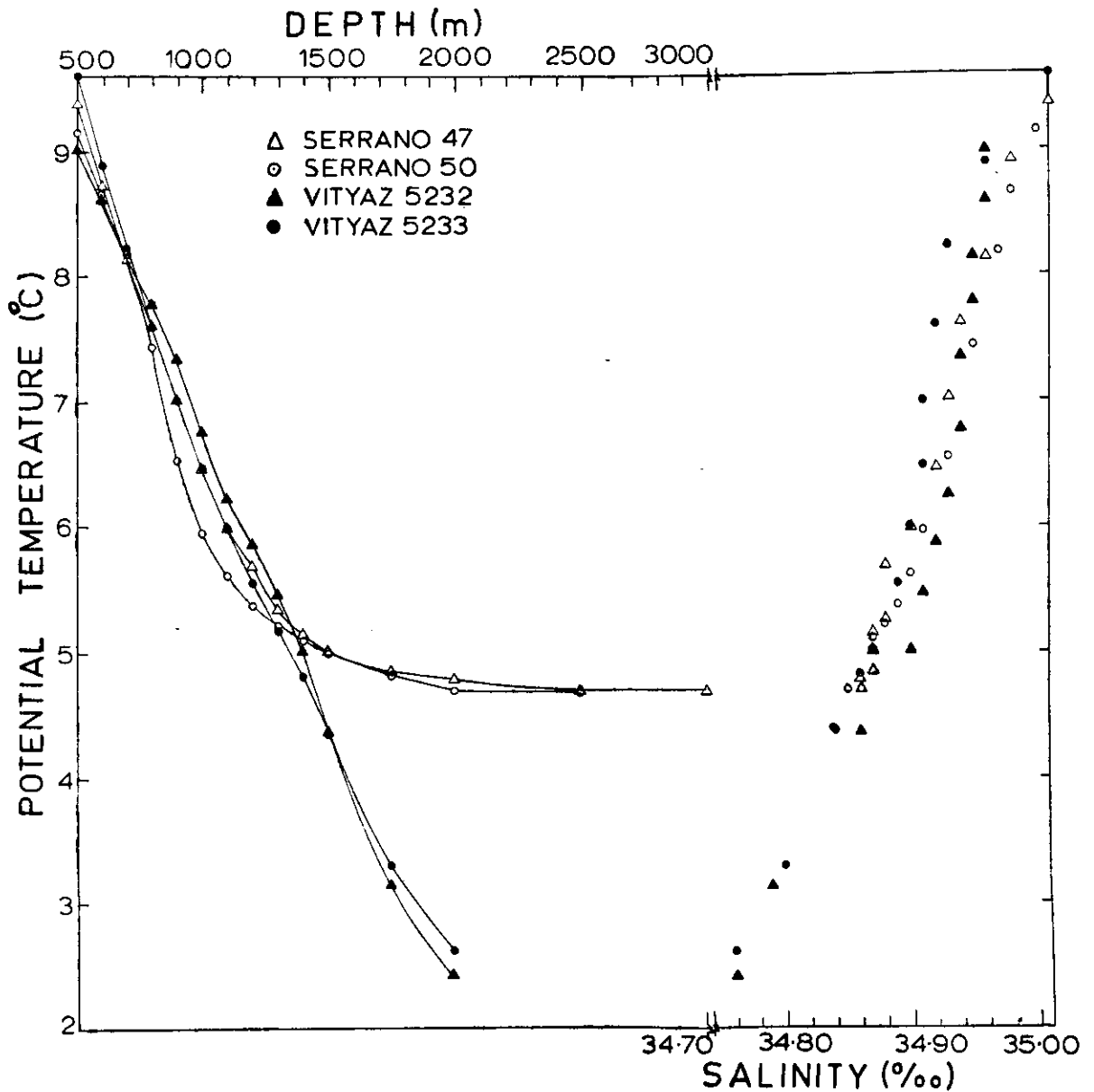
Fig. 10 — Relationship showing potential temperature versus depth and salinity
