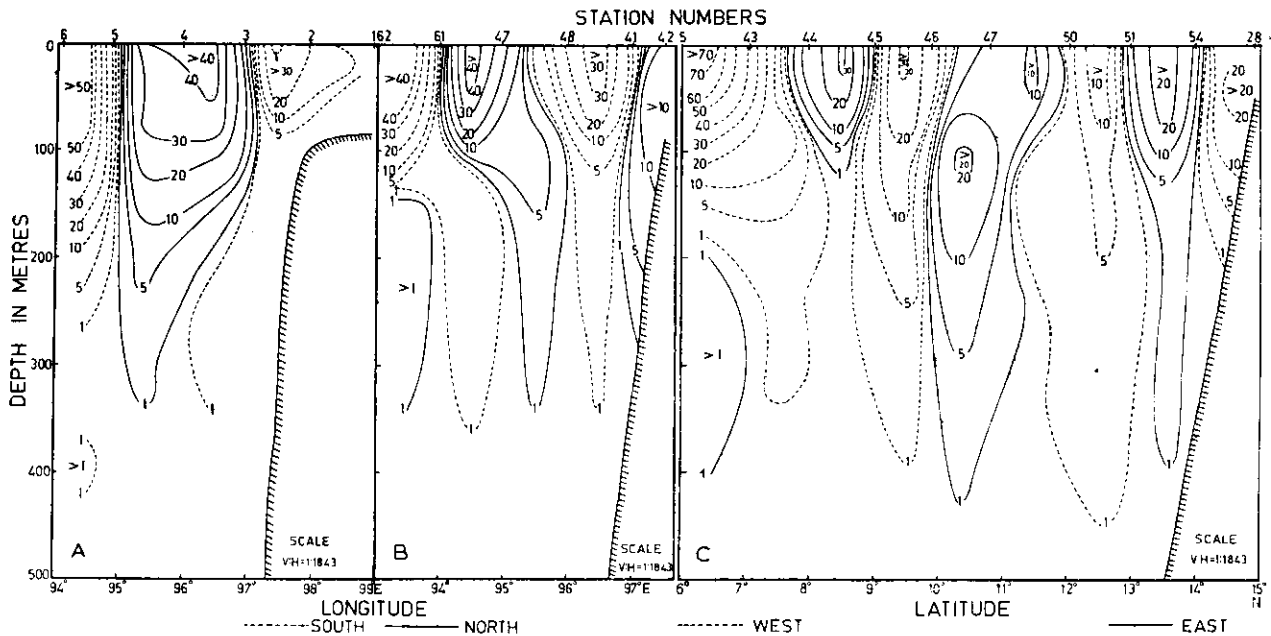
Fig. 9 — Geostrophic currents along section I (A), section II (B) and section IV (C)
