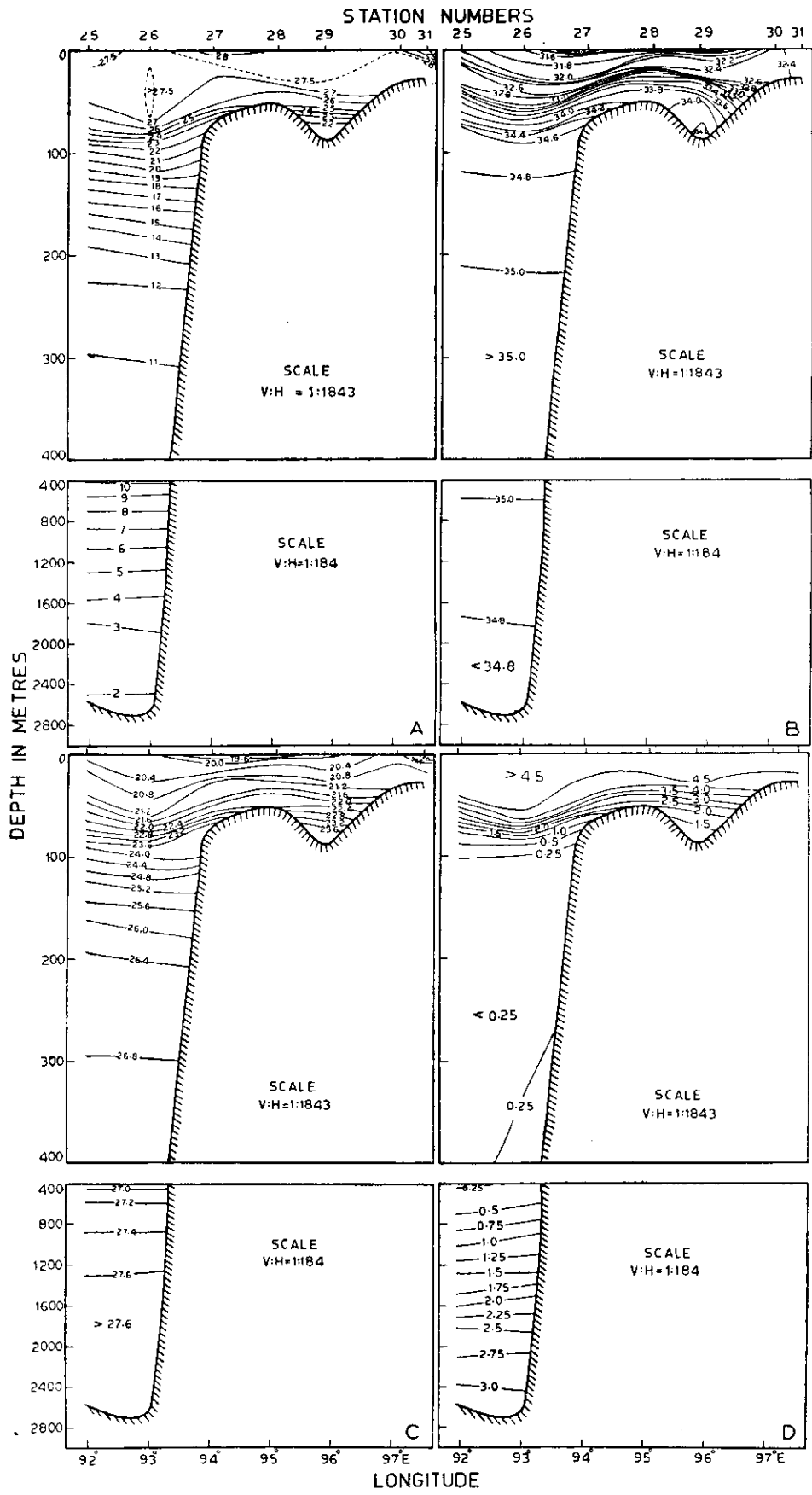
Fig. 4 — Temperature (A), salinity (B), density (C) and dissolved oxygen (D) along approximately 15°N (section III)
