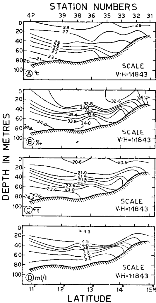
Fig. 6 — Distribution of (A) temperature, (B) salinity, (C) density and (D) dissolved oxygen along 97°30' (section V)
