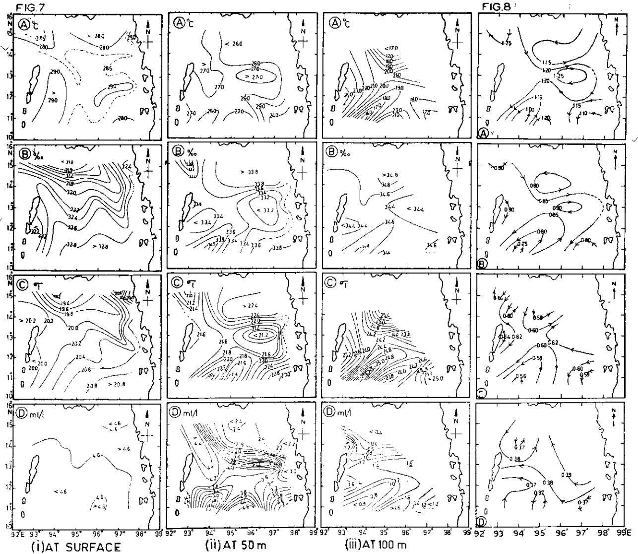
Fig. 7 — Distribution of (A) temperature, (B) salinity, (C) density and (D) dissolved oxygen at (i) surface, (ii) 50 m and (iii) 100 m
