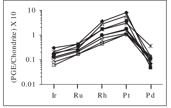
Figure 2. CI Chondrite-normalized PGE patterns of the Afanasiy–Nikitin seamount Fe–Mn crusts.
