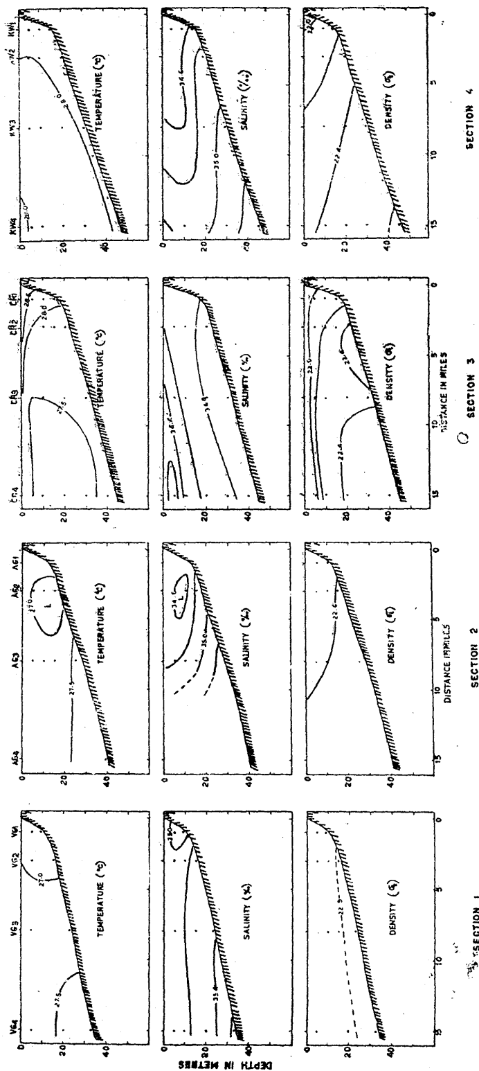
Fig. 3 Vertical distribution of temperature, salinity and density ( \sigma_t ) during Feb-March.
