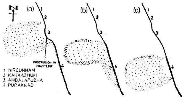
Fig. 8 -- Diagrammatic representation of the southern movement of mud bank: [a, initial location of the mud bank; b, extension of the suspended mud towards south; and c, new position of the mud bank. Periphery of the mud bank is shown by closely placed smaller dots]
