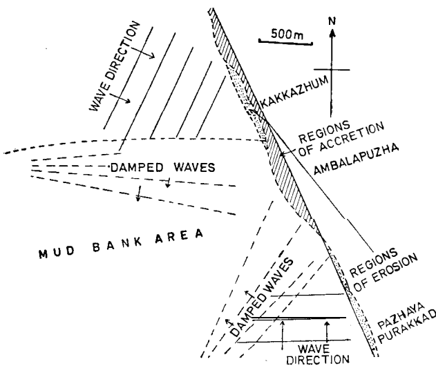
Fig. 12 -Shoreline changes induced by the presence of mud bank near Ambalapuzha during 1972 [Both southern and northern areas adjacent to mud bank get eroded, but the erosion is severe on the southern side, probably because of the proximity of a seawall nearby. Wave directions have been shown by large arrows. Damped waves within the mud bank are indicated by smaller arrows]
