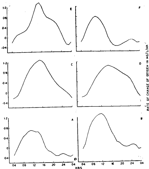
Fig. 2. Community metabolism curves
