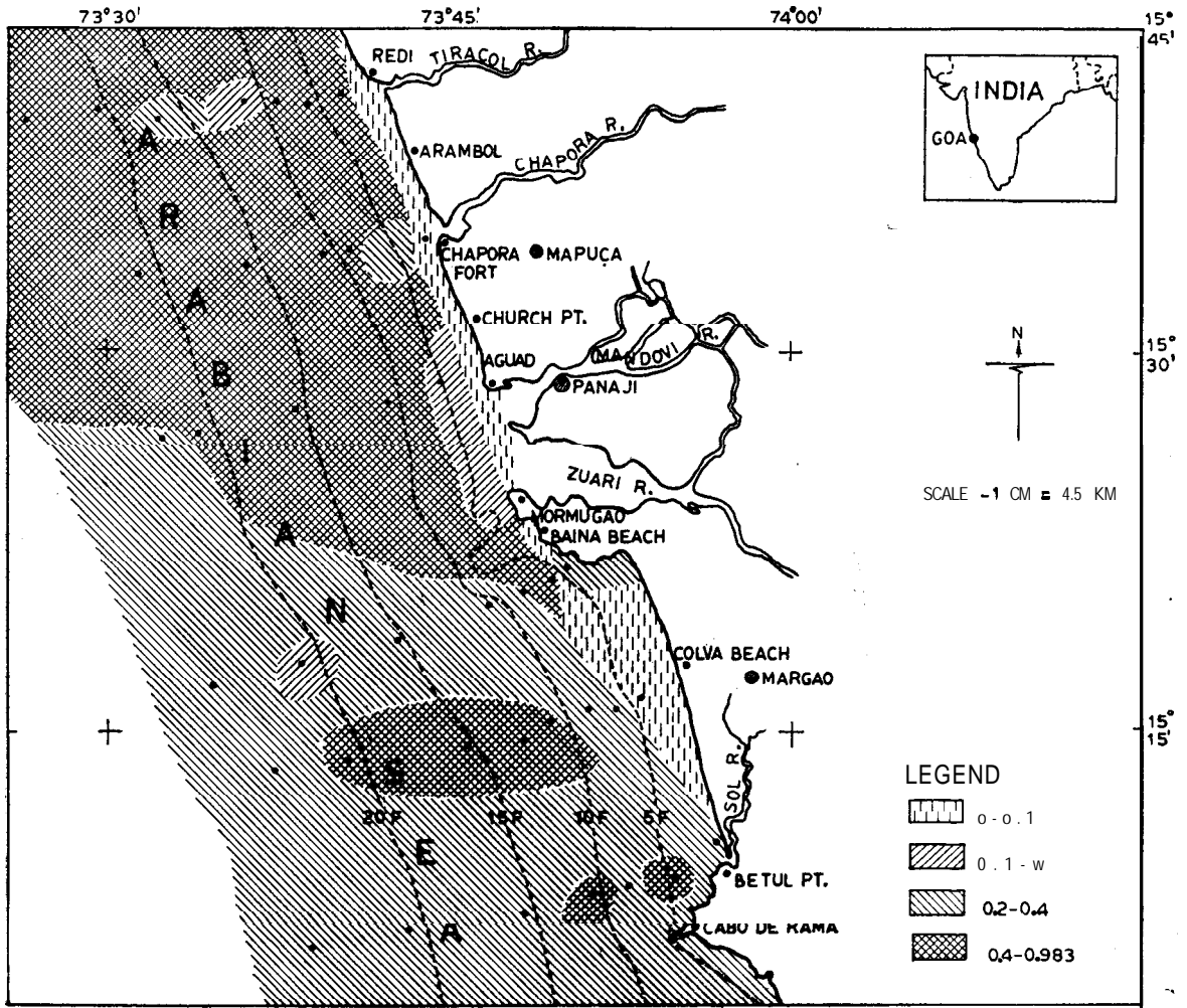
Fig. 2 — Station locations and distribution pattern of phosphorus in the nearshore sediments of Goa coast
