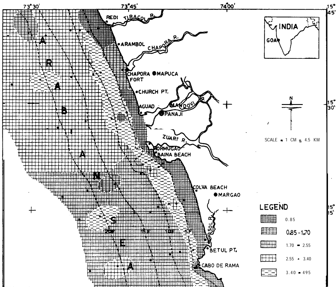
Fig. 1 — Station locations and distribution pattern of organic carbon in the nearshore sediments of Goa coast
