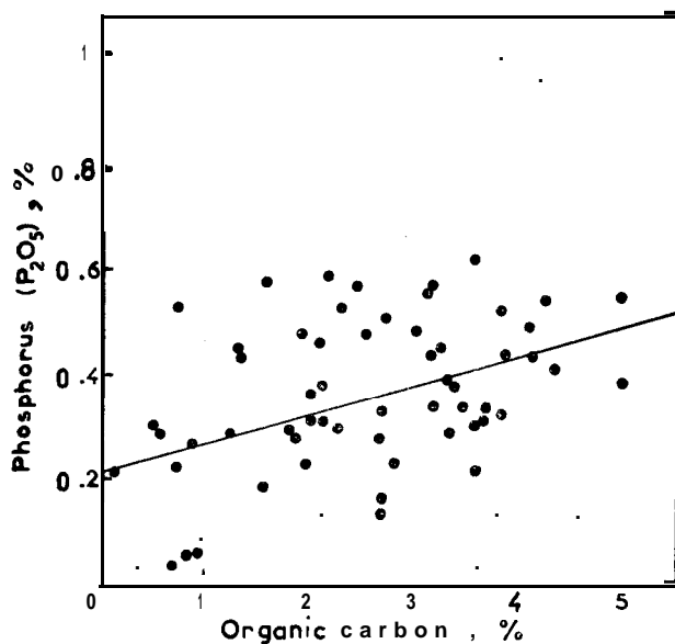
Fig. 3 — Scatter plot with least squares fit between organic carbon and total phosphorus
