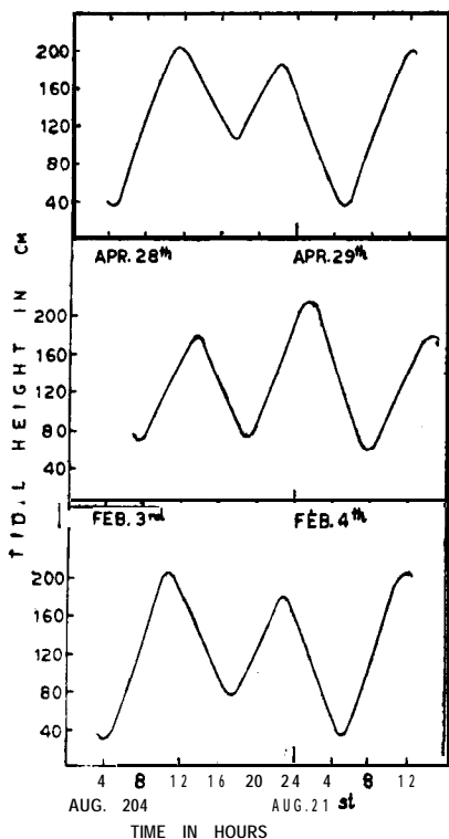
Fig. 2 — Tidal cycle in the estuary during different periods (August 1971 and February and April 1972)
