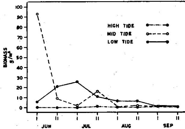
Fig. 3. Changes in the biomass (in \text{g/m}^2 ) at different tide levels.
