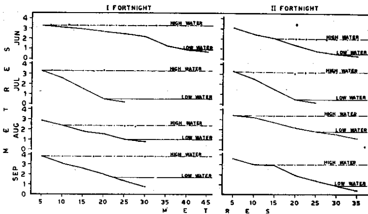
Fig. 2. Fortnightly beach profiles from June to September.
