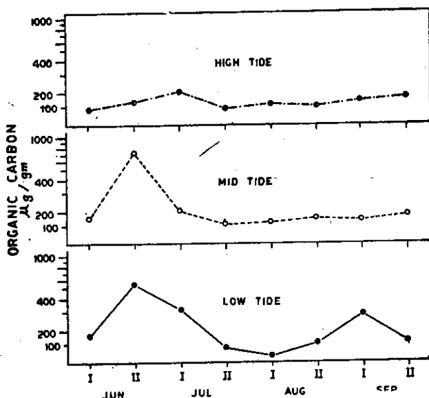
Fig. 4. Fluctuations of organic carbon in the sand at different tidal levels.
