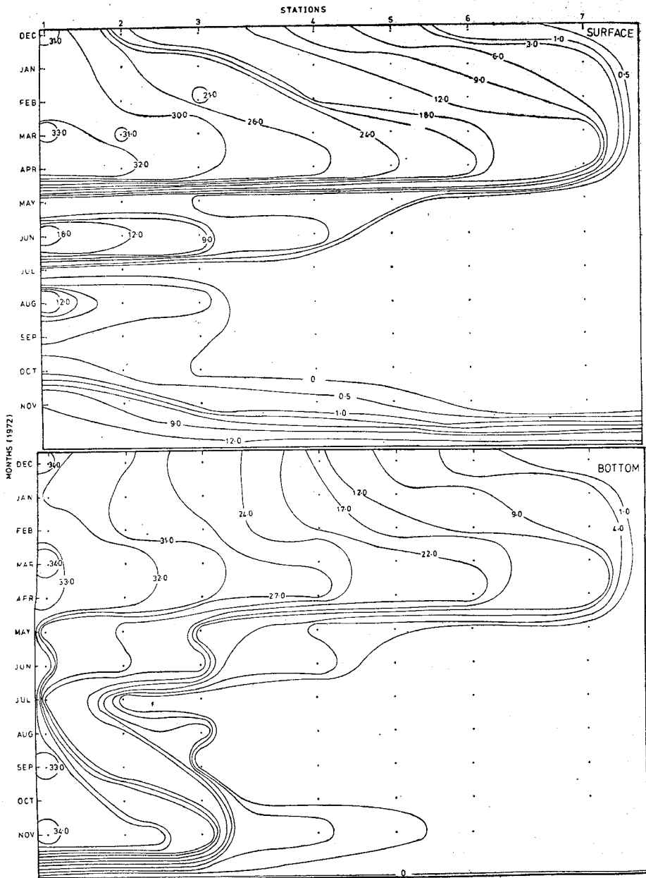
Fig. 2 — Distribution of salinity along the surface and bottom from Cochin to Alleppey during 1972
