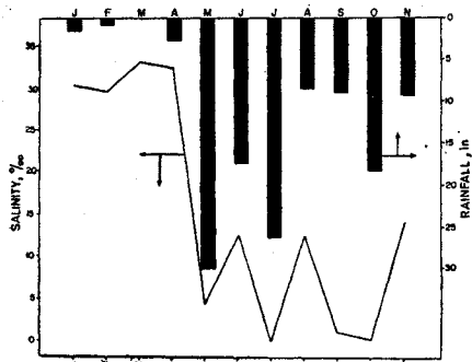
Fig. 3 — Correlation of the fluctuations in surface salinity and rainfall at station 1 during 1972
