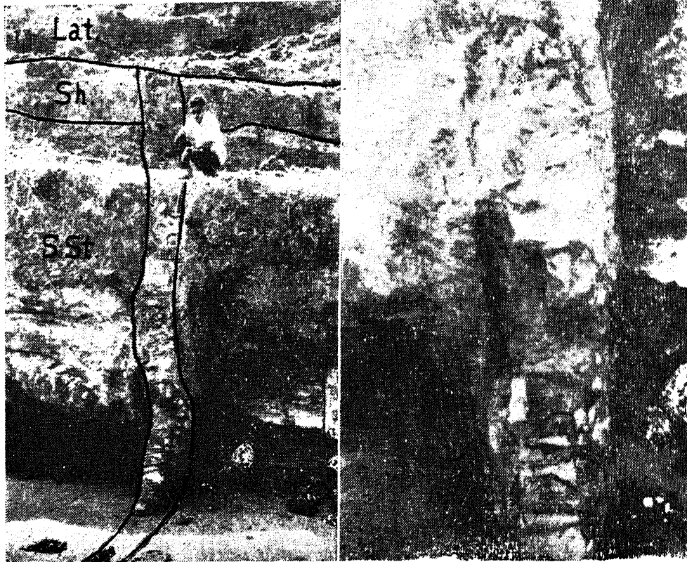
FIG. 1. Clastic dike intrusive into sandstone-shale sequence at Baga, Goa.
