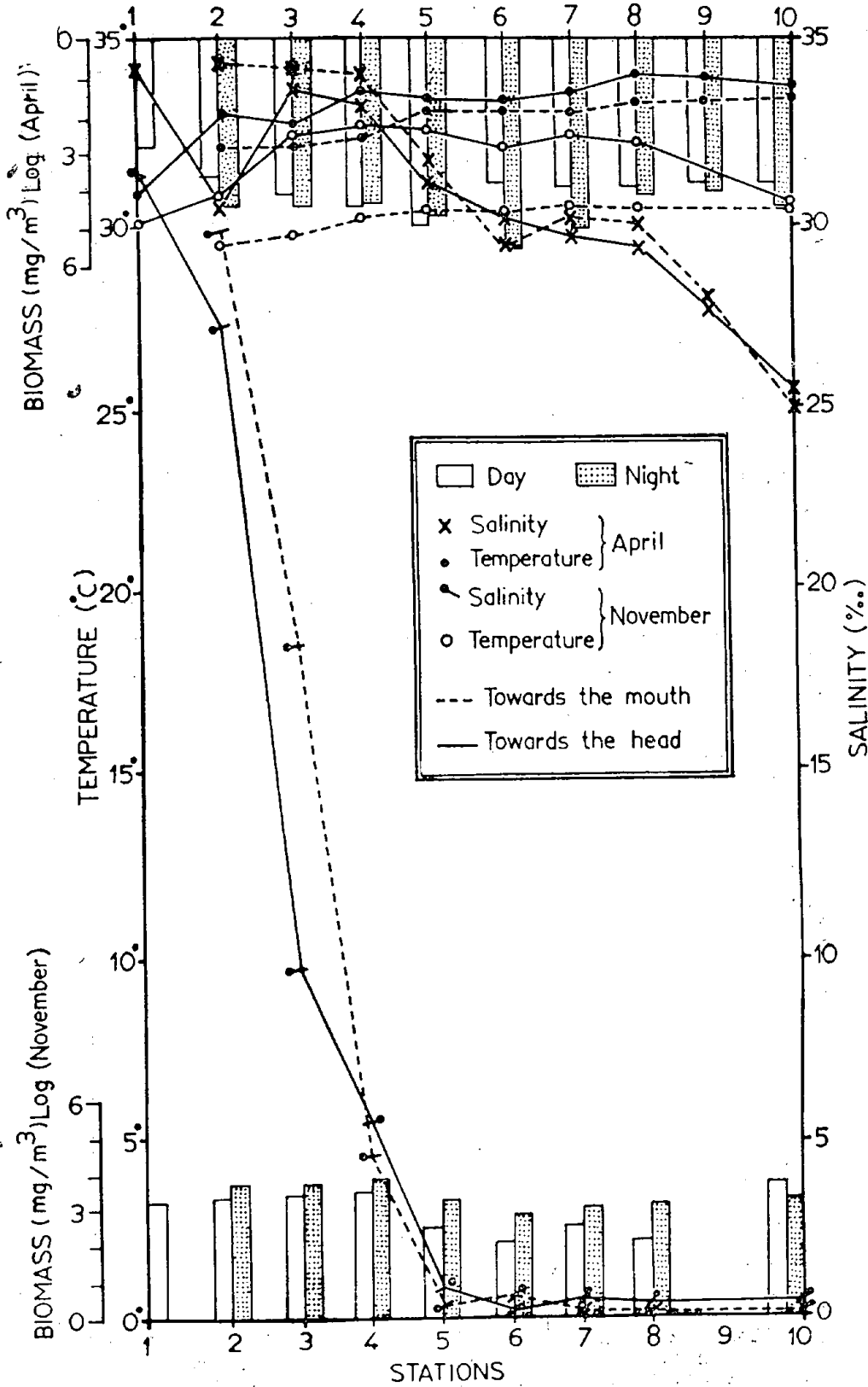
FIG. 2. Surface temperature (°C), salinity (‰) and biomass (mg/m³) at stations between Fairway buoy and Alleppey during November and April.
