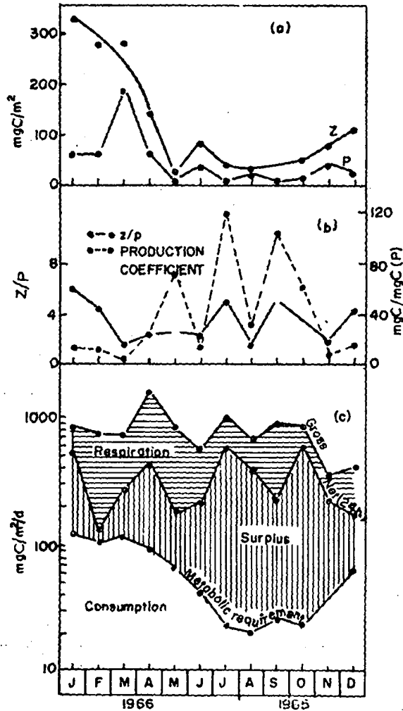
FIG. 11. (a) Relation between phytoplankton (P) and zooplankton (Z) taken from parallel hauls on the same day. (b) Relation between zooplankton: phytoplankton ratio (Z/P) and production coefficient (Photosynthesis: carbon content of phytoplankton). (c) Relation between metabolic requirement of zooplankton and gross and net (24 hrs) primary production. The lower portion shows the approximate consumption of primary production by zooplankton herbivores; the middle portion shows the approximate surplus of basic food and the upper portion shows the average respiration (24 hrs).
