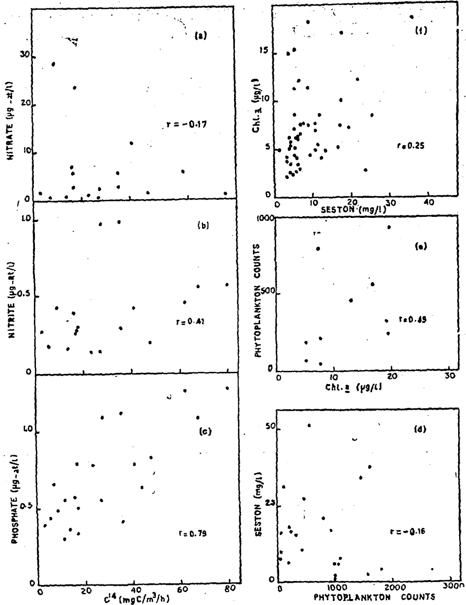
FIG. 8. The relation between net primary production ( C^{14} ), nutrients, phytoplankton counts, seston and chlorophyll; 'r' denotes the correlation coefficient.
