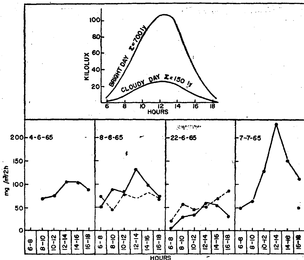
FIG. 3. Diurnal variations in the photosynthetic activity in each of the four experiments; C^{14} uptake (solid lines), net O_2 production (broken lines). Top figure shows two extreme conditions of diurnal illumination.
