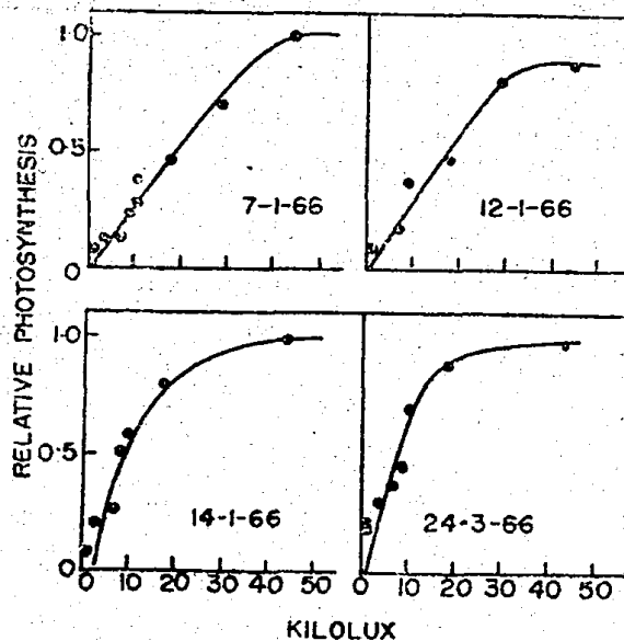
FIG. 4. The relation between photosynthesis and light intensities in surface phytoplankton. Each curve refers to a different experiment.
