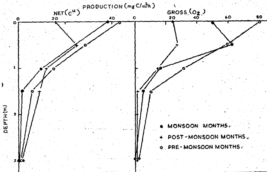
FIG. 6. Gross and net primary production in three seasons in relation to depth.
