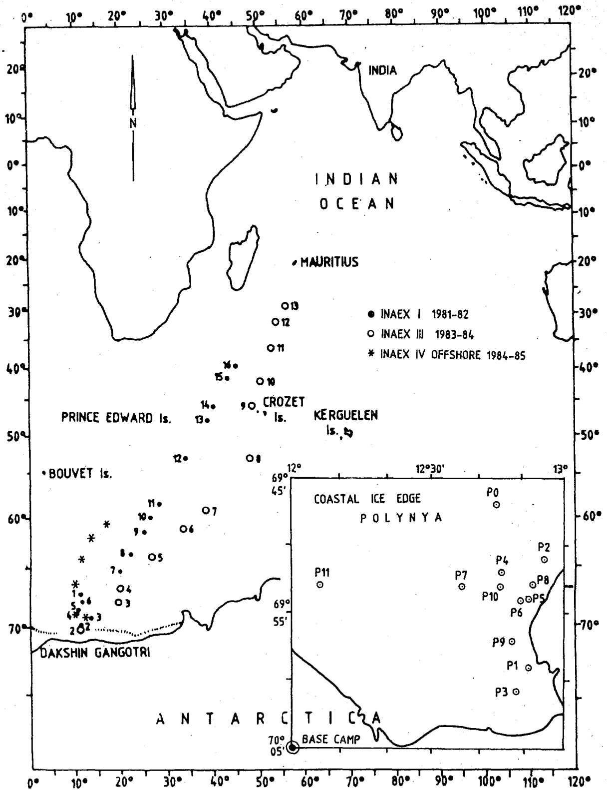
Fig. 1. Station position during I, III and IV Antarctic Expeditions (INAEX I, III & IV). Inset shows the position of the stations in the ice shelf region (P 0 to P 11 ) during INAEX IV.
