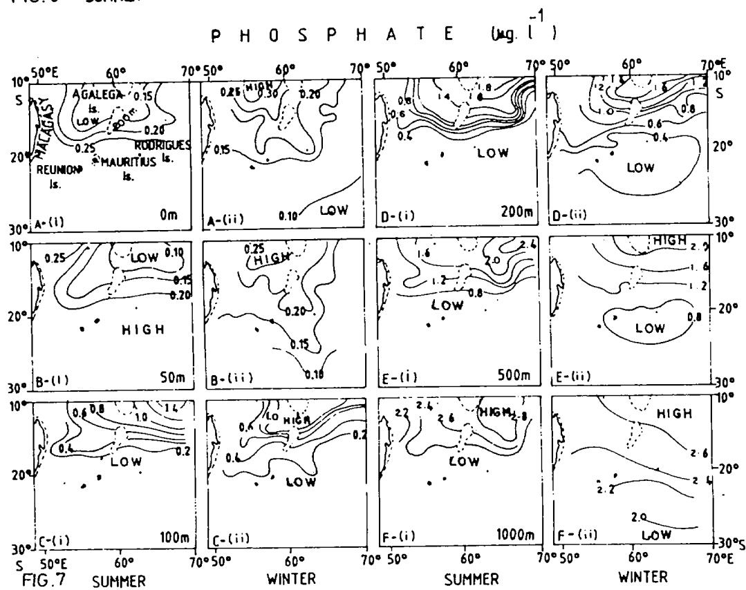
Fig. 6 - Distribution of oxyty at (A) surface (B) 50 (C) 100 (D) 200 (E) 500 and (F) 1000 m during summer (i) and winter (ii) Fig. 7 - Distribution of inorganic phosphate at (A) surface (B) 50 (C) 100 (D) 200 (E) 500 and (F) 1000 m during summer (i) and winter (ii)
