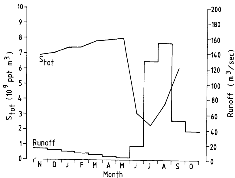
Figure 5. Annual cycles of S_{\text{tot}} (see equation (1)) and monthly-mean run off ( \text{m}^3/\text{sec} ).
