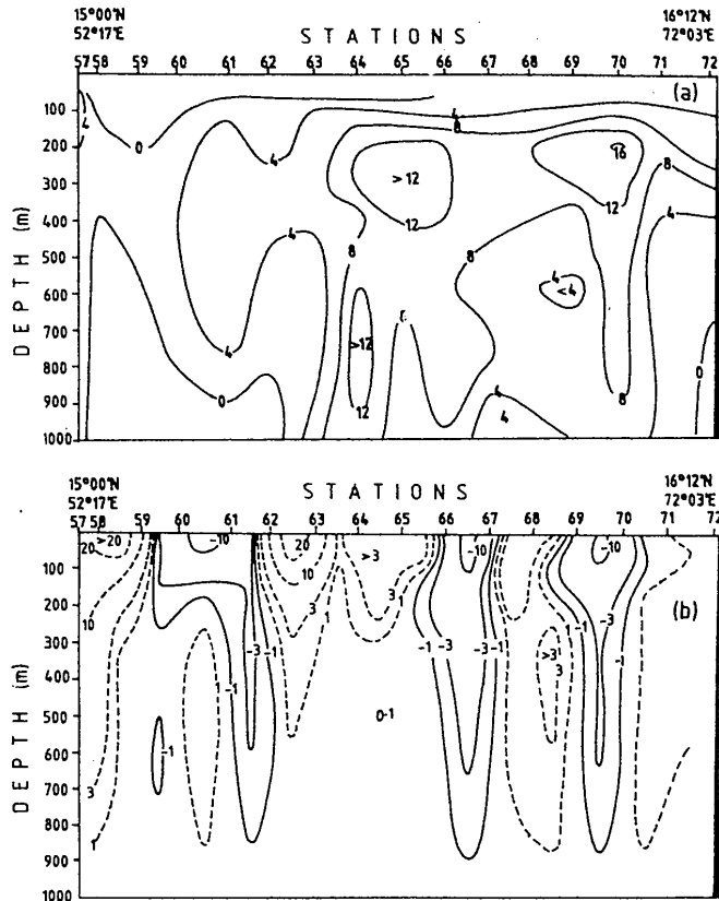
Figure 8. (a) Distribution of nitrate deficits ( \mu\text{g-at. dm}^{-3} ) in Section III ( Atlantis II HIOE data); and (b) Relative barocline currents ( \text{cm s}^{-1} ) in Section III computed with 1,000-db surface as the reference level: solid lines—southerly flow; broken lines—northerly flow.
