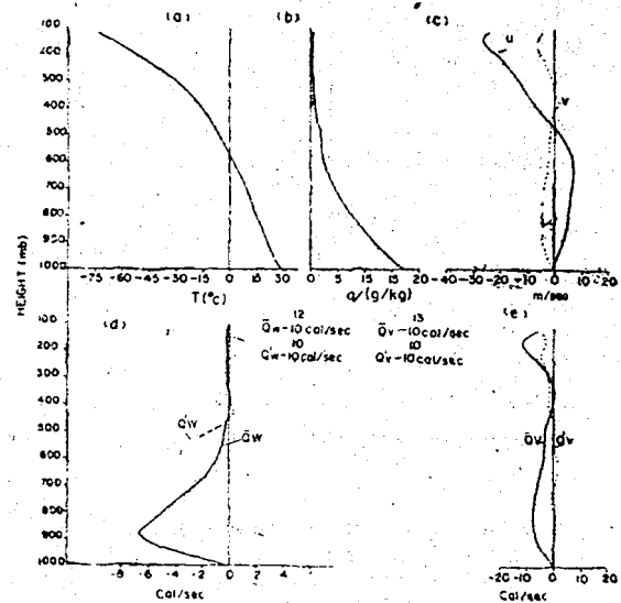
Fig. 5. Same as Fig. 2 but for southern boundary wall
