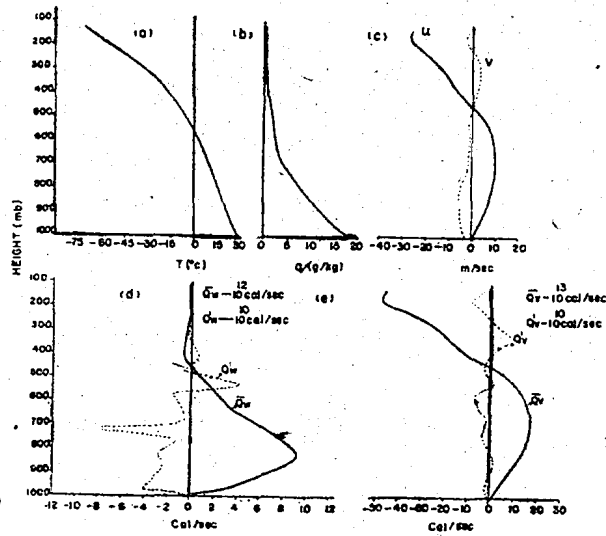
Fig. 3 Same as Fig. 2 but for western boundary wall
