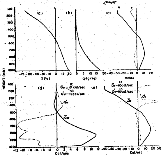
Fig. 2. Mean profiles of temperature ( \bar{T} ), specific humidity ( \bar{q} ), wind components ( \bar{u} & \bar{v} ), lateral flux of latent heat ( \bar{Q}_w & \bar{Q}'_w ), and dry static energy ( \bar{Q}_v & \bar{Q}'_v ) across eastern boundary wall
