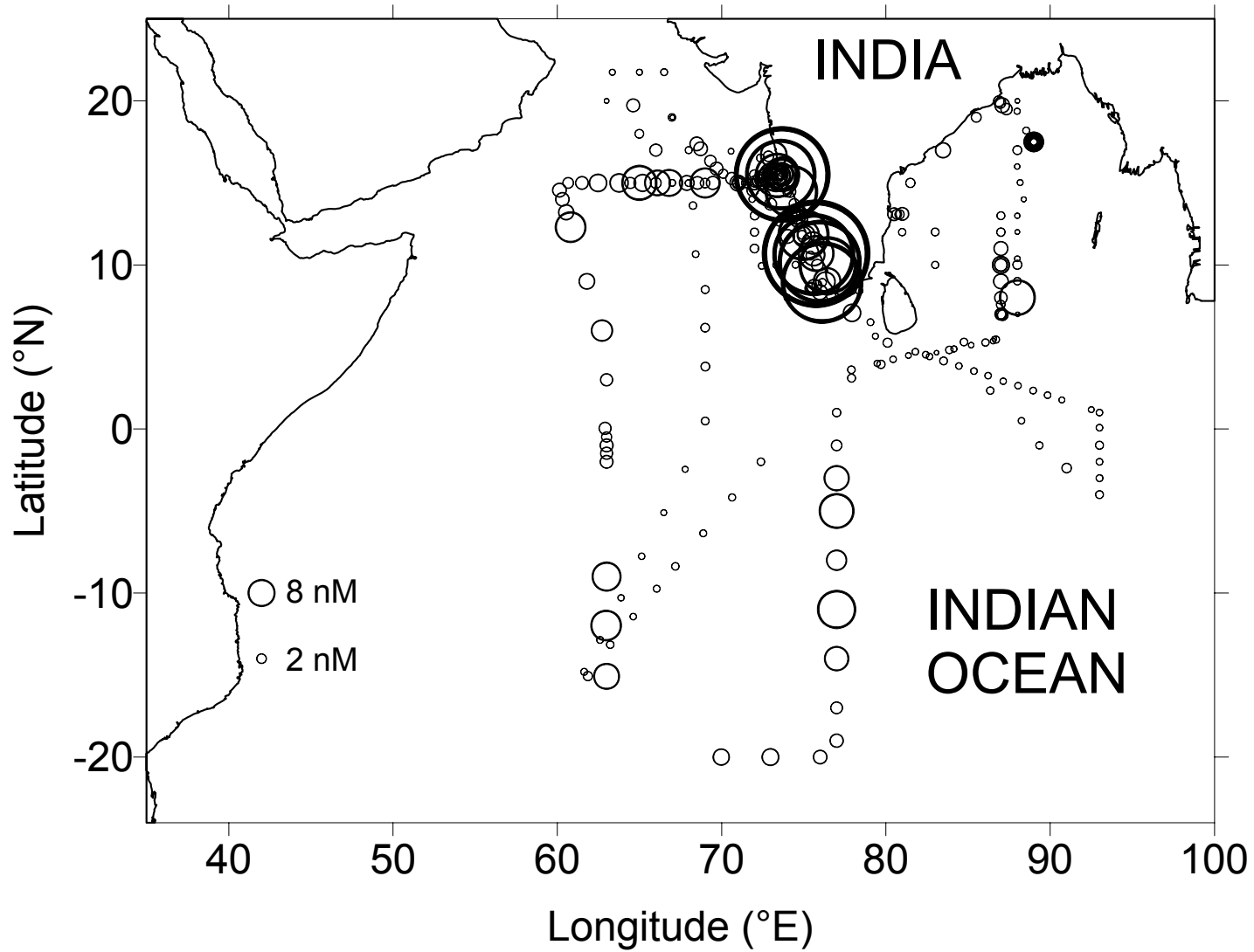
Figure 11. Variations in surface DMS concentration in the Indian Ocean. Maximum concentration of 525 nM found in the coastal waters of Goa is not shown here.
