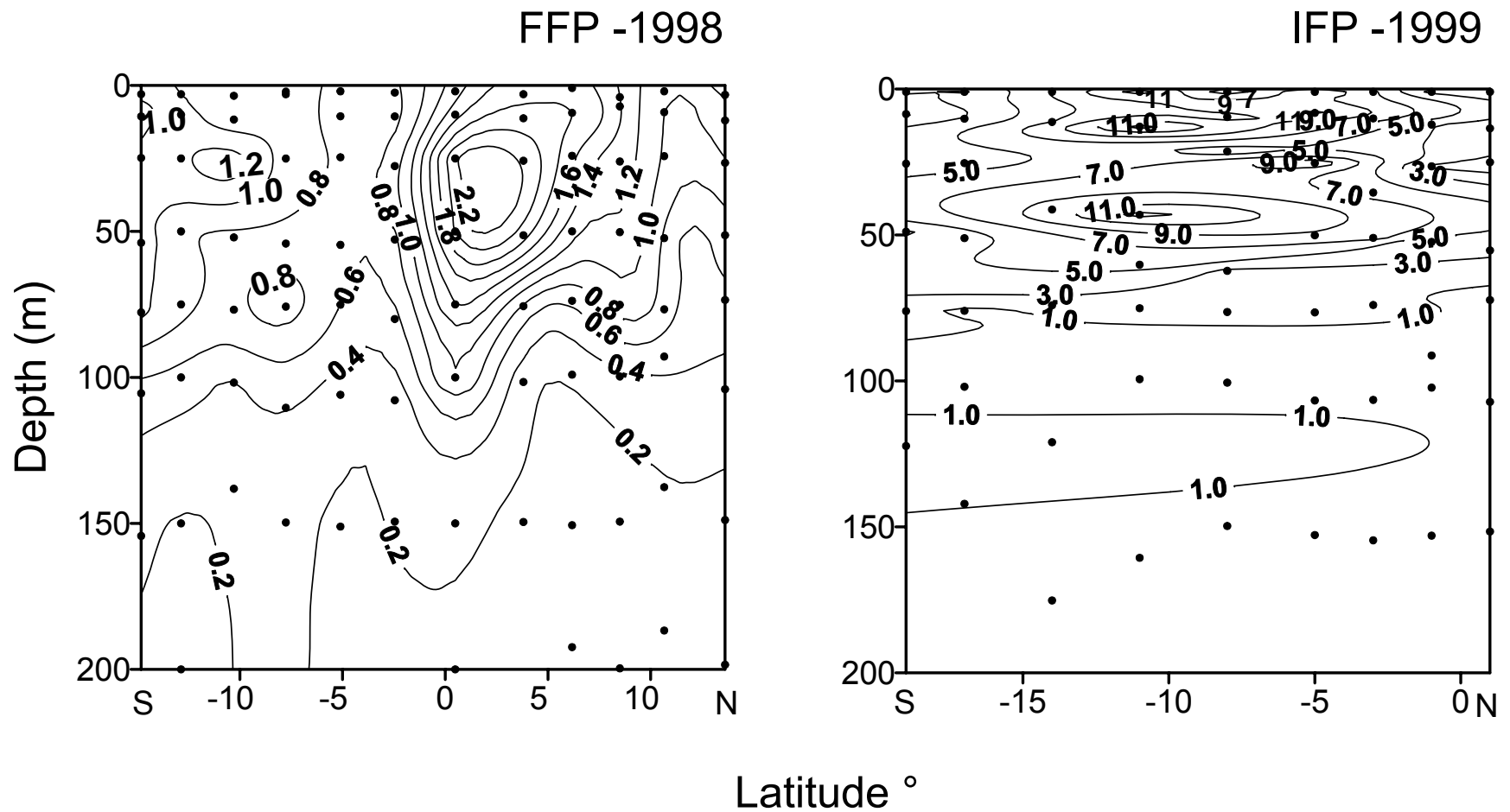
Figure 7. Variations in DMS (nM) in the Central Indian Ocean in winter season of 1998 (FFP; SK133) and 1999 (IFP; SK141) of the INDOEX project.
