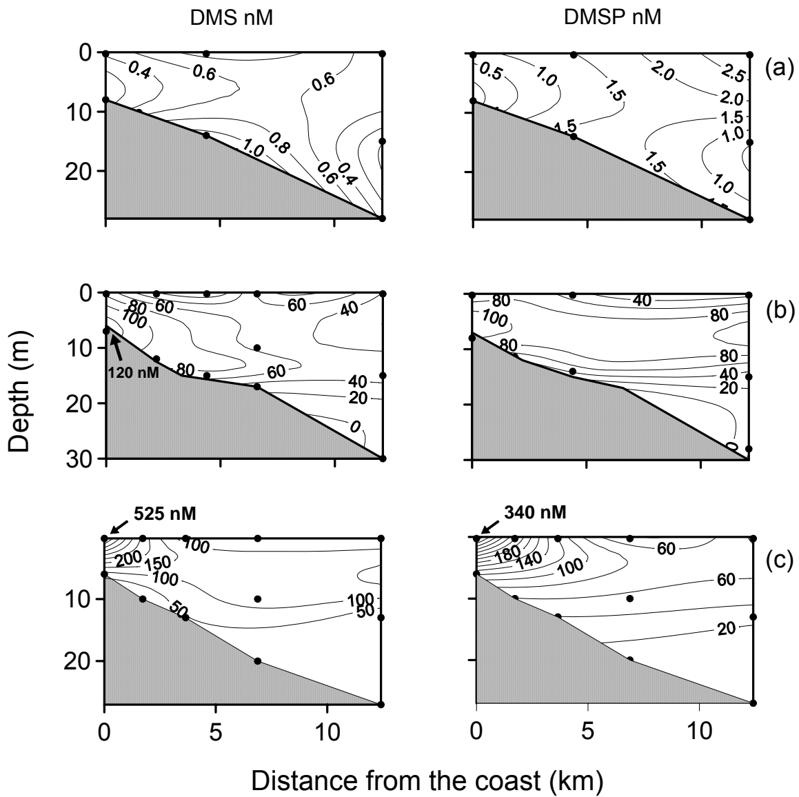
Figure 10. Time series observations of DMS (Left panels) and DMSP_t (Right panels) off Candolim in Goa on (a) 28/3/2001, (b) 29/9/2000 and (c) 11/11/1999.
