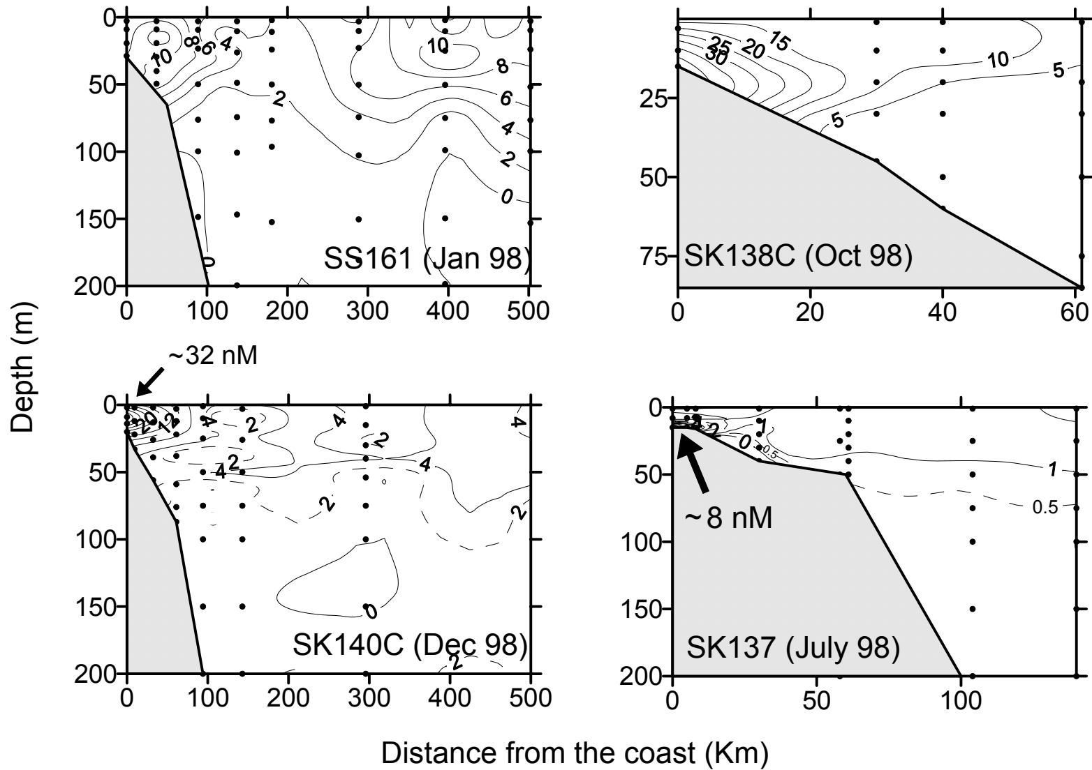
Figure 5. Longitudinal variations in DMS off Goa in different seasons.
