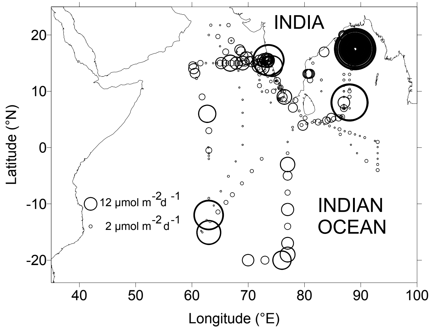
Figure 12. Variations in DMS flux in the Indian Ocean. Time series station (SK147A & B) in the Bay of Bengal depicts wide variations in the DMS flux.
