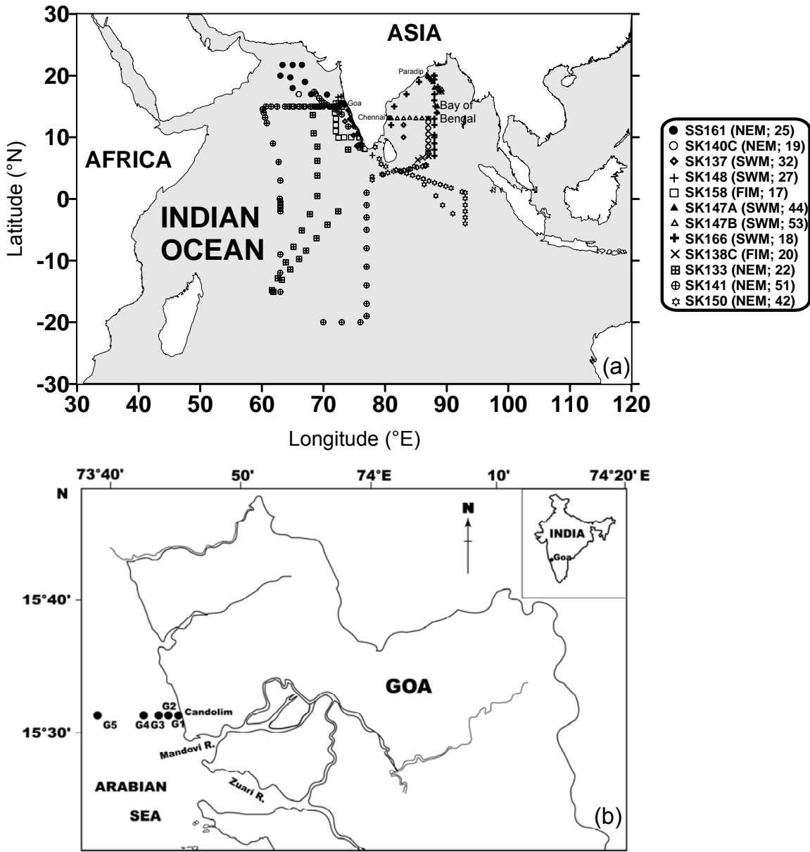
Figure 1. a) Station locations occupied for dimethyl sulphide studies in the central and north Indian Ocean. Symbol index indicates cruise number, season and number of stations. b) Station locations off Candolim, Goa.
