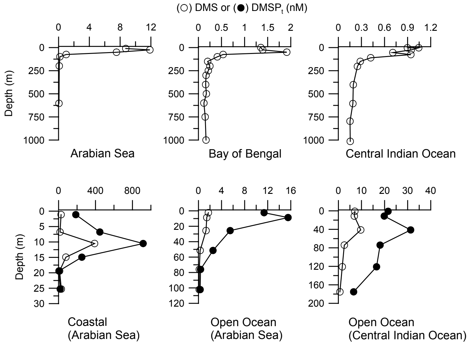
Figure 4. Typical vertical profiles of DMS and DMSP t in different regions of the Indian Ocean.
