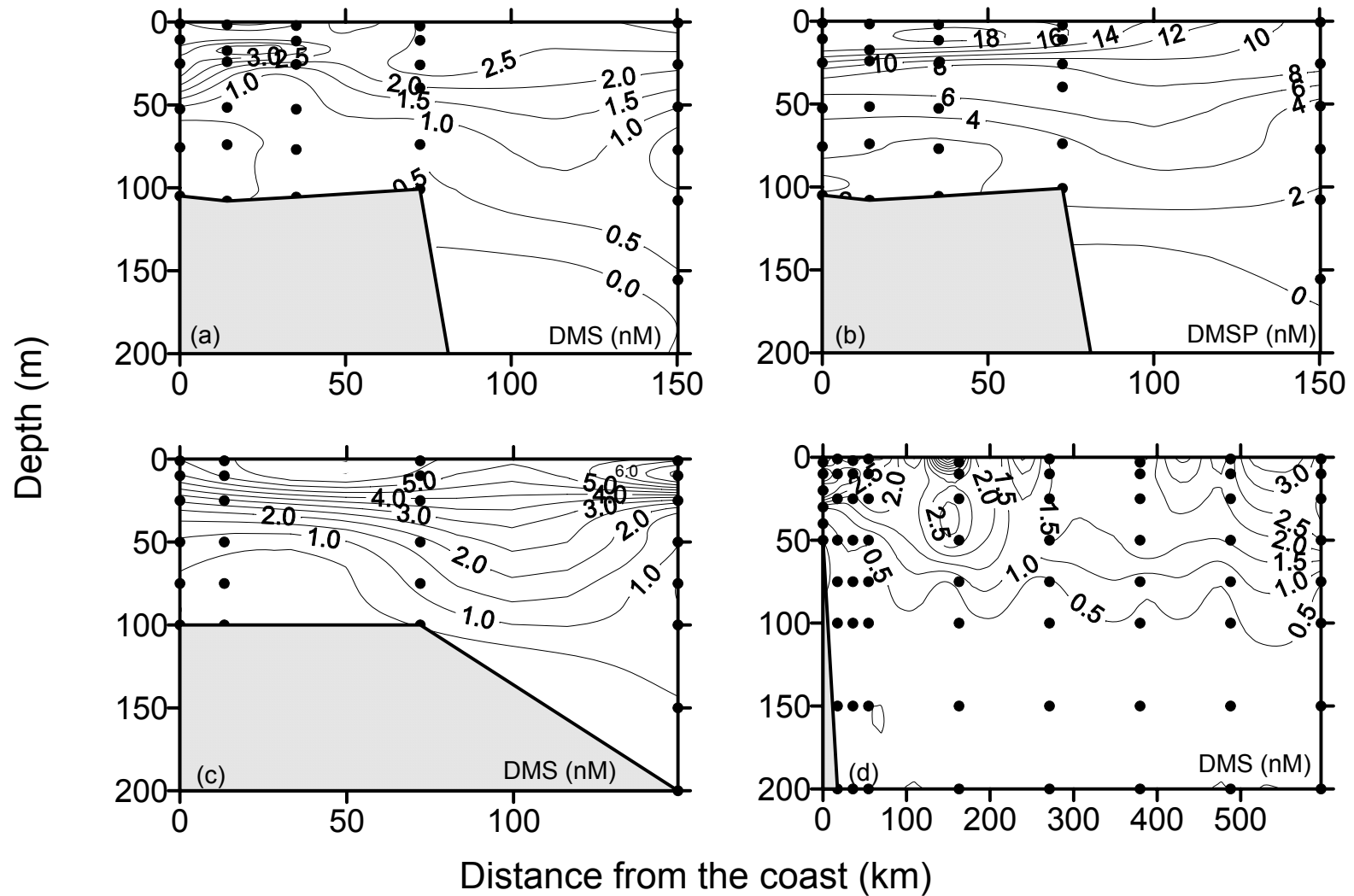
Figure 6. Variations in DMS and DMSP_t off Paradip (a) and (b) during SK147A and (c) during SK147B and off Chennai (d) during SK147B.
