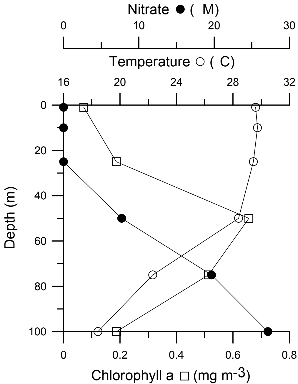
Figure 3. Profiles of temperature, nitrate and chlorophyll (at 9.94°N, 72.44°E, SK158) showing subsurface chlorophyll maximum.
