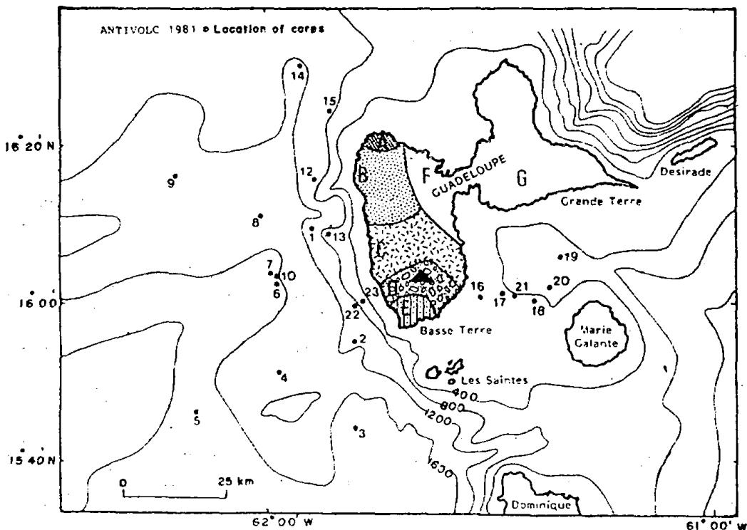
Fig. 1. Location of cores collected in the Guadeloupe archipelago. The geology of the island is represented as A-Hornblende andesites; B-Calc-alkaline rocks, dacites and andesites; C-Acid andesite flows; D-Recent calc-alkaline rocks with hypersthene and augite. Solid triangle represents "La Soufriere" active volcano; E-Olivine basalts; F-Altered zone; G-Calcareous deposits of marine origin (Data from Westercamp and Mervoyer, 1976).
