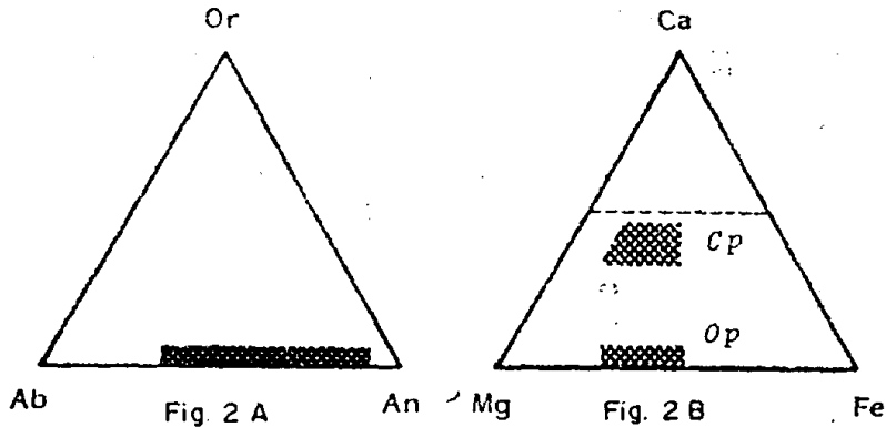
Fig. 2. Or-Ab-An (A) and Ca-Mg-Fe (B) diagrams showing the position of plagioclase and pyroxene group of minerals resp. (Op: orthopyroxenes; Cp: clinopyroxenes.)
