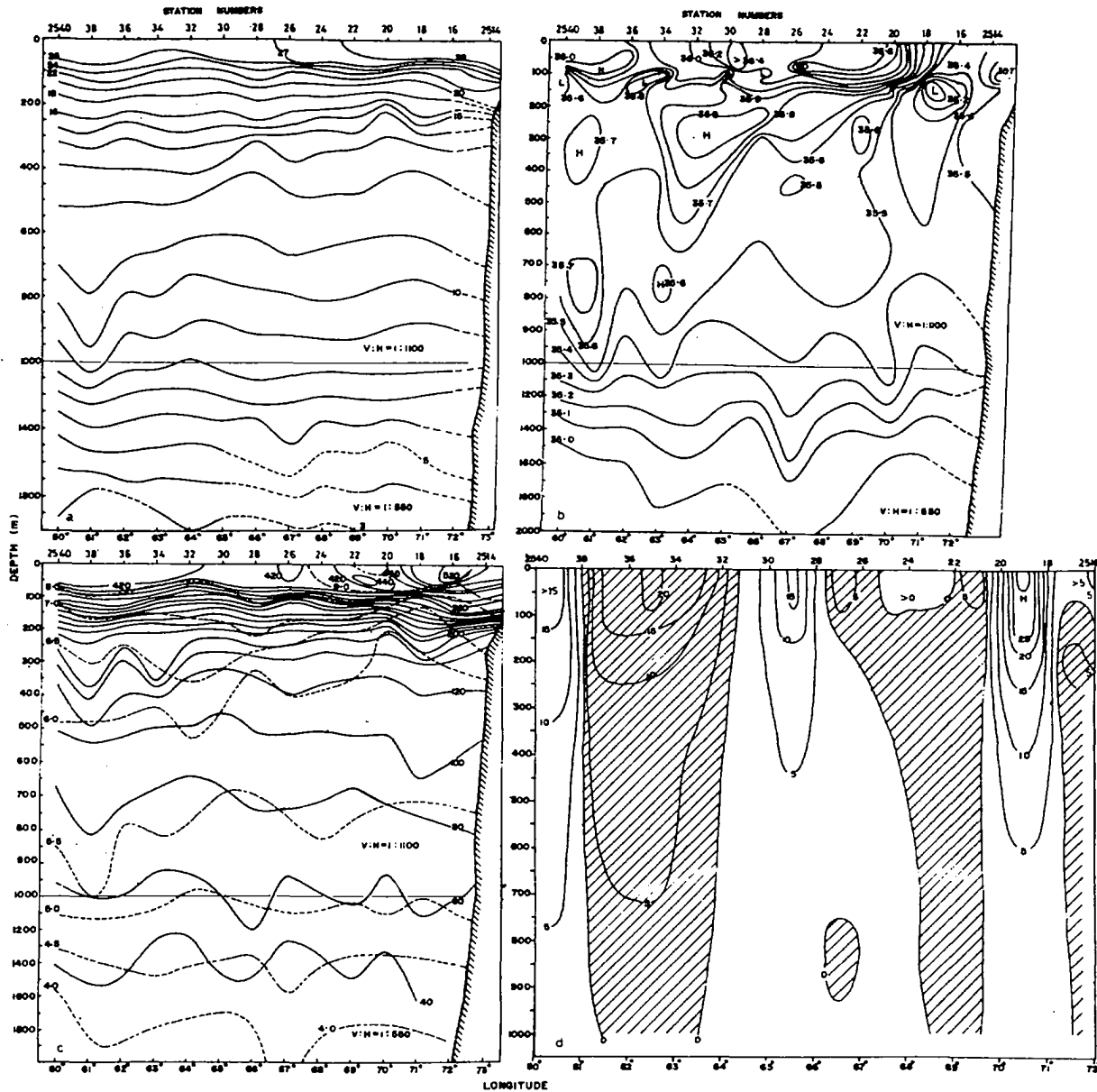
Fig. 2 – Vertical (a) thermal structure, (b) salinity structure, (c) thermocline anomaly distribution and density flux function, and (d) geostrophic current structure along 15^{\circ}\text{N}
