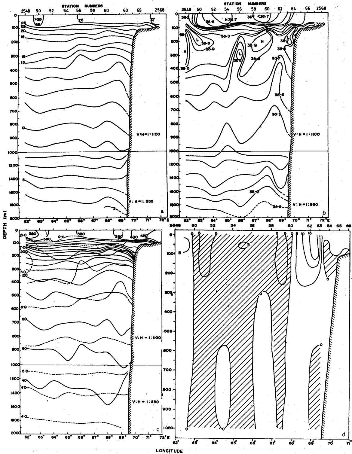
Fig. 3 - Vertical (a) thermal structure, (b) salinity structure, (c) thermocline anomaly distribution and density flux function and (d) geostrophic current structure along 19°N
