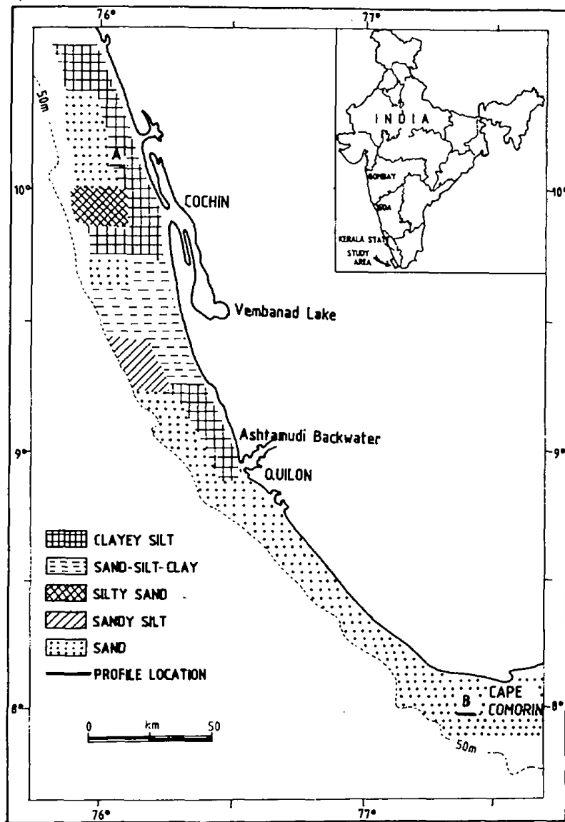
Figure 1. Surface sediment texture. Note the distinct difference in texture, north and south of Quilon.
