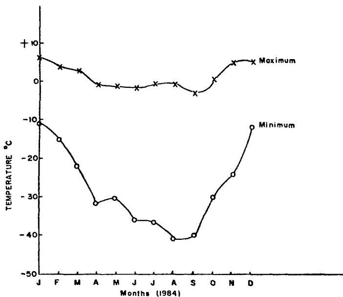
Fig. 2. Temperature cycle in Oasis.
