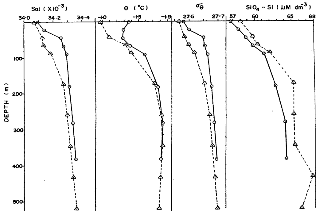
Fig. 2a Vertical profiles of salinity, potential temperature ( \theta ), potential density ( \sigma_\theta ) and silicate-silicon at the shelf station occupied on 11th January (circles) and 7th February (triangles)
