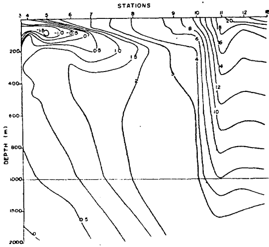
Fig. 3 Vertical section of potential temperature ( ^{\circ}\text{C} ) between 68^{\circ}30'\text{S} , 19^{\circ}55'\text{E} and 29^{\circ}43'\text{S} , 54^{\circ}34'\text{E}
