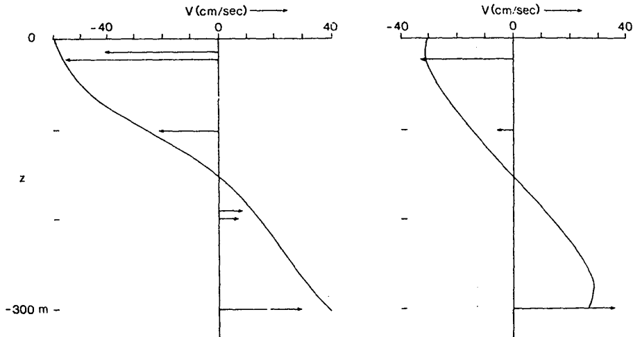
Figure 2. Observed equatorward velocity component of the currents off the west coast of Australia at 25.4S (left panel) and at 22S (right panel). The arrows are measurements from a current meter; the curve from geostrophy using 150 m as a level of no motion. The undercurrent is nearly as strong as the surface flow. The Leeuwin Current strengthens to the south. (After Thompson, 1984).
