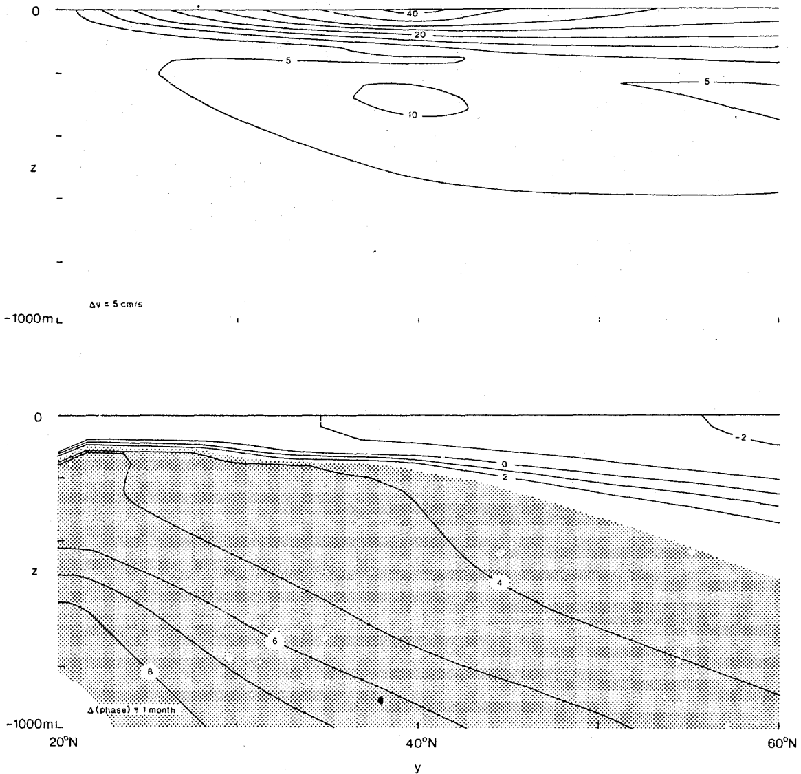
Figure 9. A meridional section at x = -8 km showing the amplitude and phase (in months) of v in the upper and lower panels, respectively, when the forcing \rho_s oscillates at the annual cycle. Positive phase indicates that v leads \rho_s . The shaded region indicates where the lead has values from 3 to 9 months. At t = 0 , currents are poleward in unshaded regions and equatorward in shaded regions, and this vertical structure is very similar to the corresponding steady flow in Figure 6. There is a relative minimum in v across which phase changes rapidly, indicating that the solution has characteristics of a vertically standing wave. Phase propagates upward everywhere, however, indicating that it also looks like a vertically propagating Kelvin wave.
