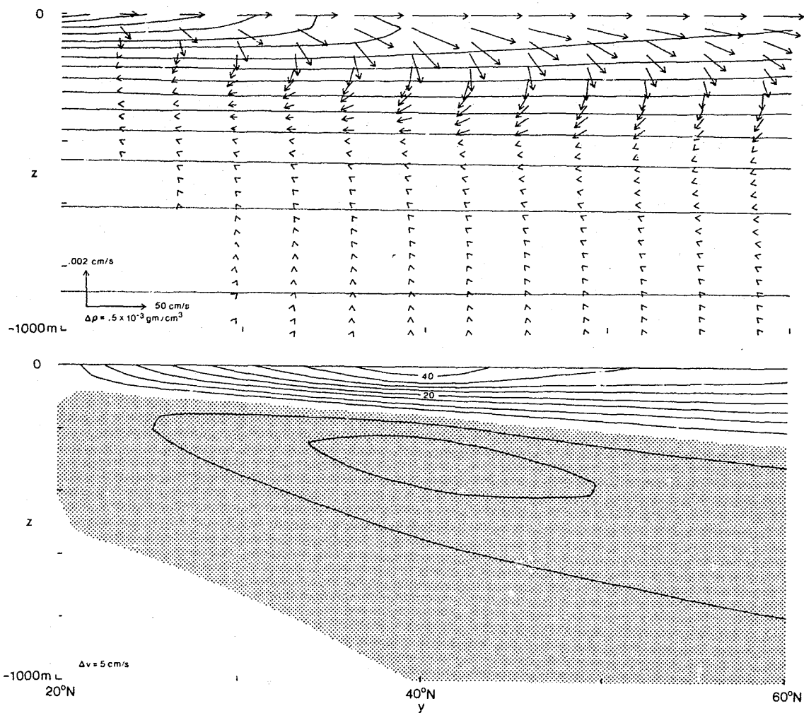
Figure 6. A meridional section showing v , w and \rho in the upper panel and contours of v in the lower panel when the forcing is a steady \rho_s . The section is located at x = -8 km, the distance offshore at which the alongshore currents achieve their maximum speeds (Fig. 5). Regions of negative (equatorward) flow are shaded. The alongshore currents increase in strength to 40\text{N} , the northern edge of the forcing region. There is a weak density inversion at the ocean surface from about 35\text{N} to 40\text{N} .
