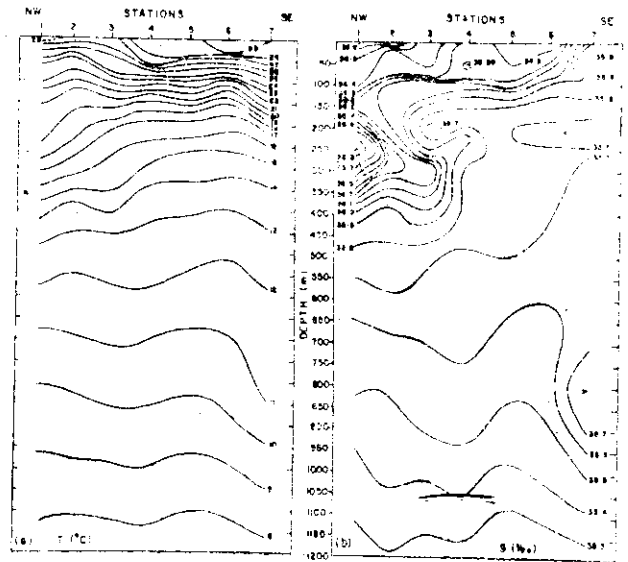
Fig. 7 (a&b). Distribution of (a) Temperature and (b) Salinity along Section IV
