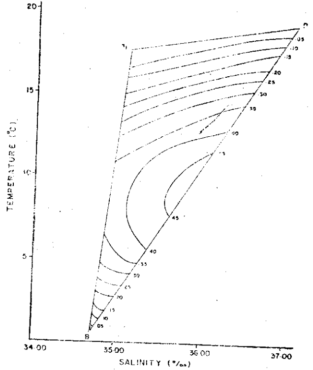
Fig. 9. Triangle of densification on mixing of Persian Gulf water (P), Hypothetical water (H 1 ) and Bottom Water (B)
