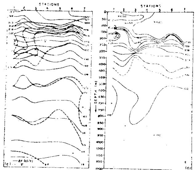
Fig. 7 (c&d). II Distribution of (c) Thermocline anomaly and density flux function and (d) Vertical stability along Section IV
