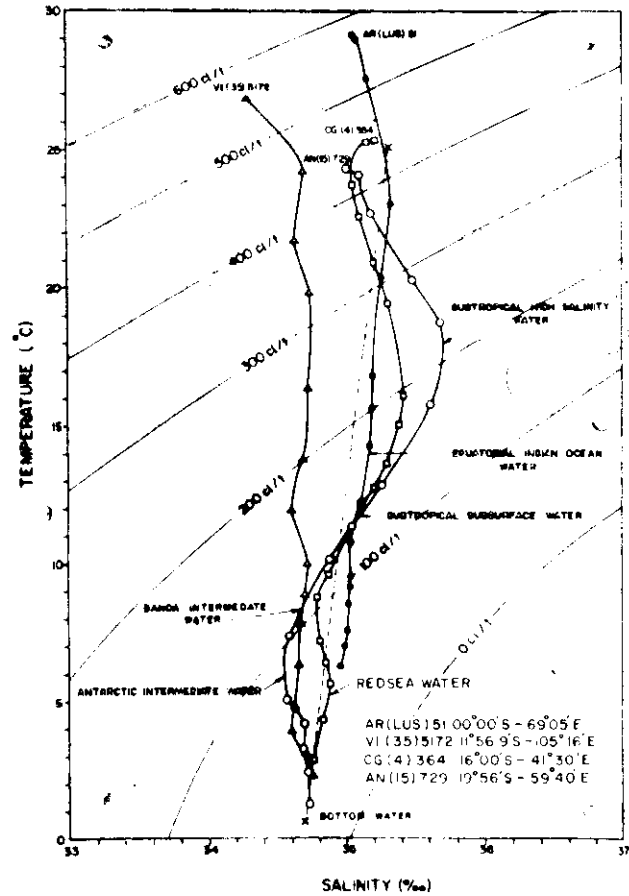
Fig. 1(b). Temperature-salinity diagrams of a few typical stations in the south Indian Ocean
