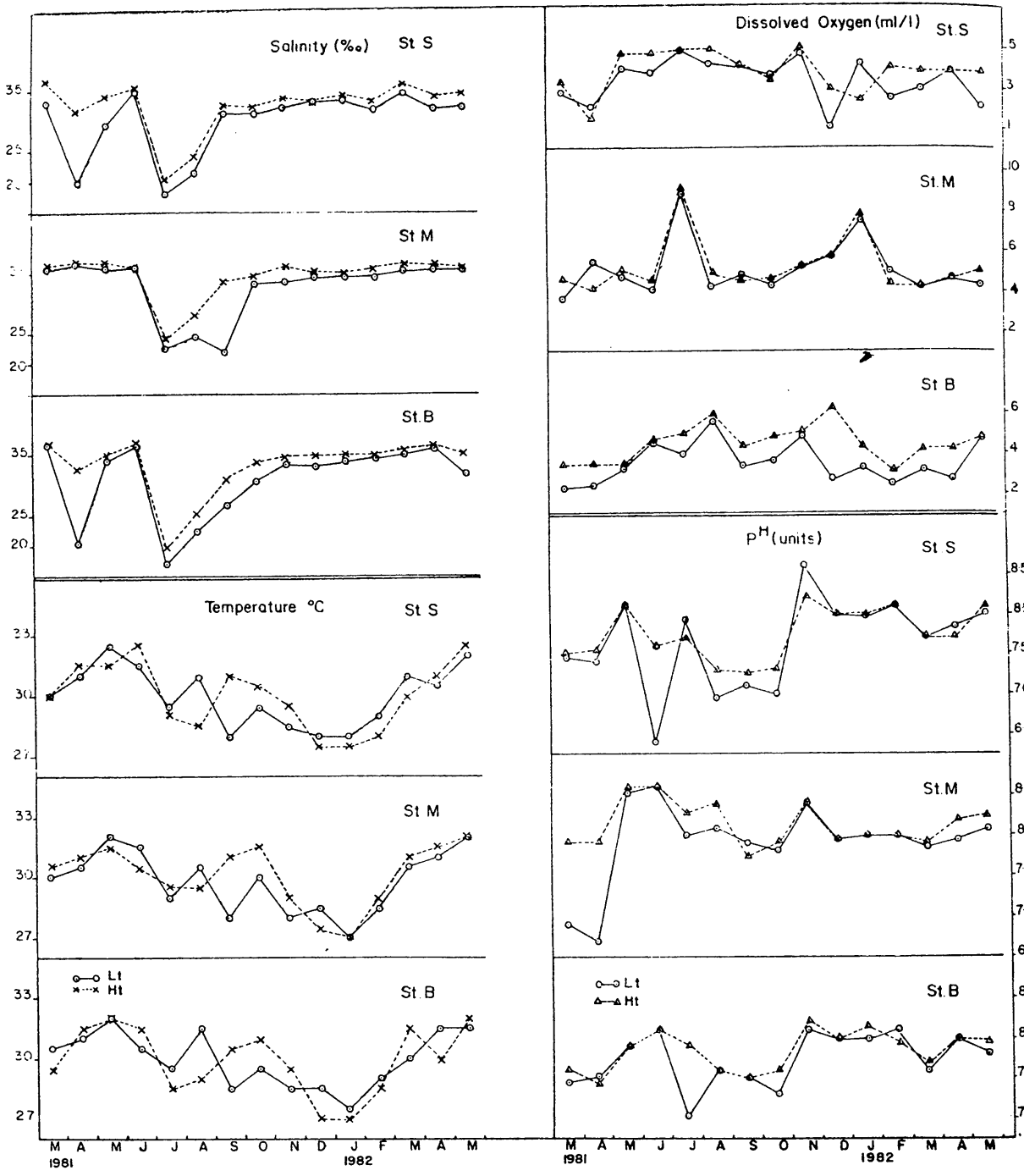
Fig. 2. Monthly fluctuations in temperature, salinity pH & dissolved oxygen for high and low tides at different stations.
