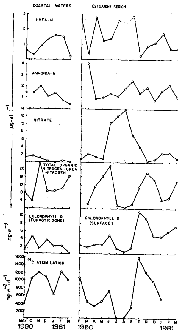
Fig. 3—Seasonal variation of integrated mean values of different parameters in coastal and estuarine waters
