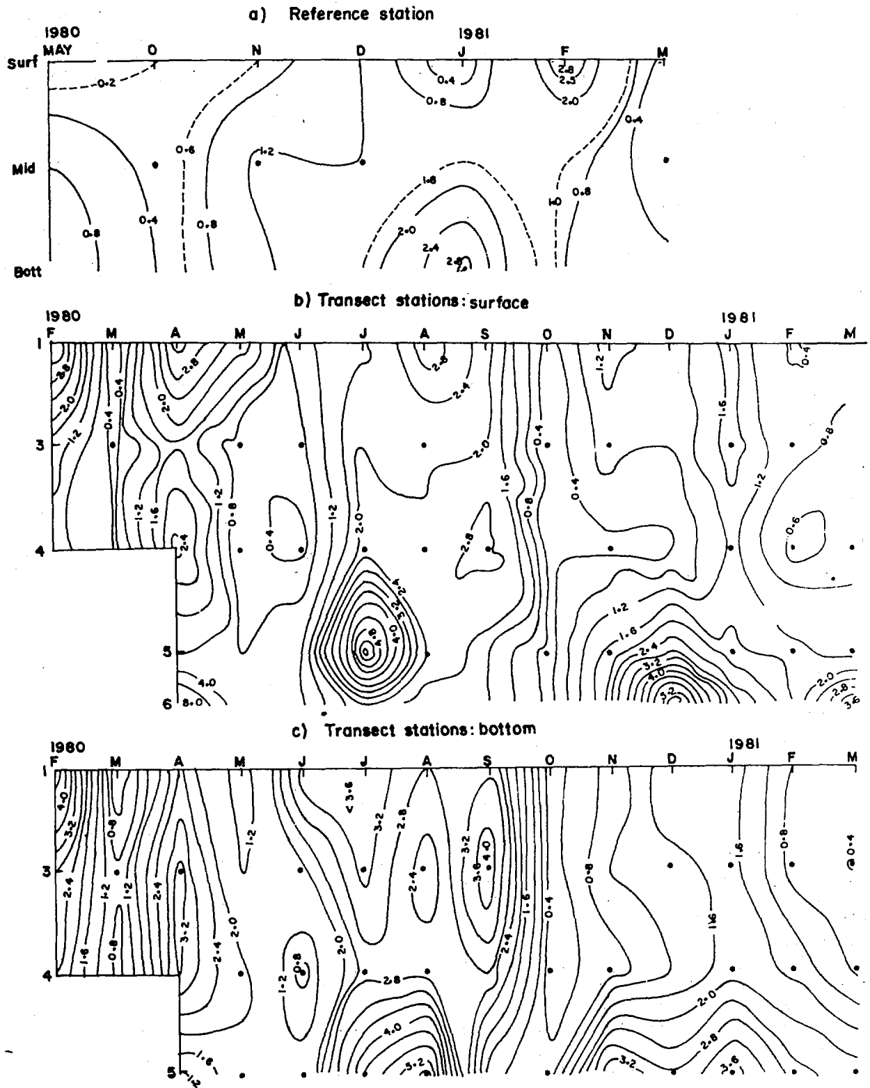
Fig. 2—Urea distribution at reference station (a) and transect survey stations (b and c)
