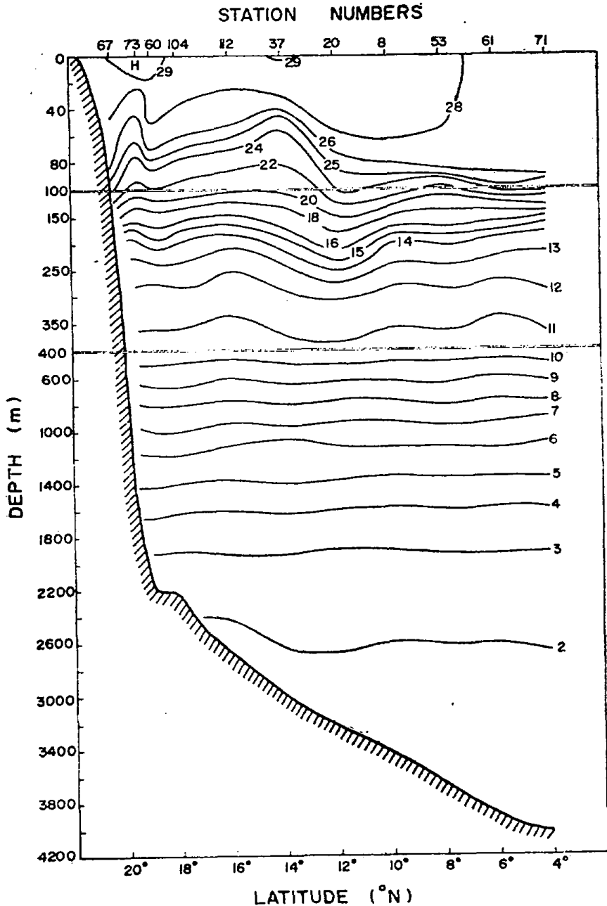
Fig. 2. Vertical distribution of temperature ( ^{\circ}\text{C} ).
