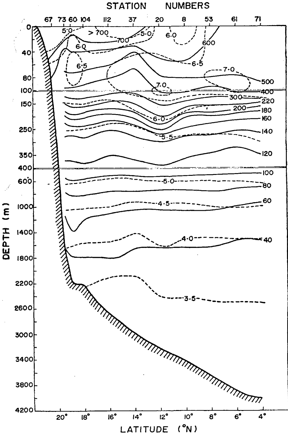
Fig. 4. Vertical distribution of thermosteric anomaly (cl/t) (solid lines) and density flux function (broken lines).
