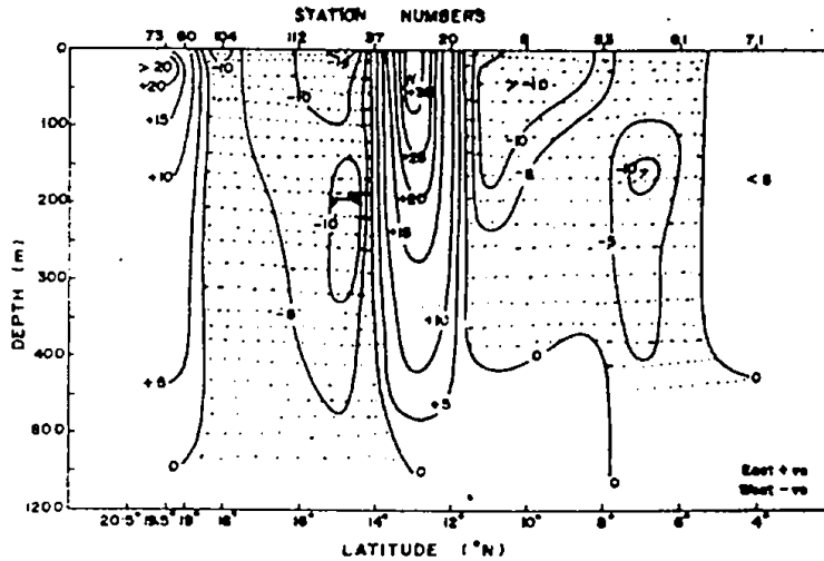
Fig. 7. Vertical current structure (cm/sec).
