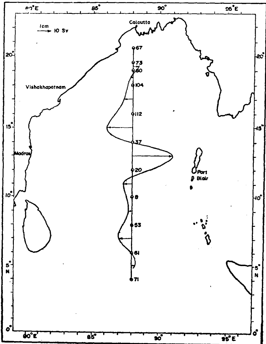
Fig. 1. Station locations and volume transport (Sverdrups).
