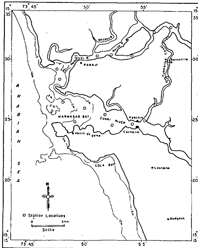
Fig. 1 — Mandovi-Zuari-Cumbarjua estuarine complex of Goa.
