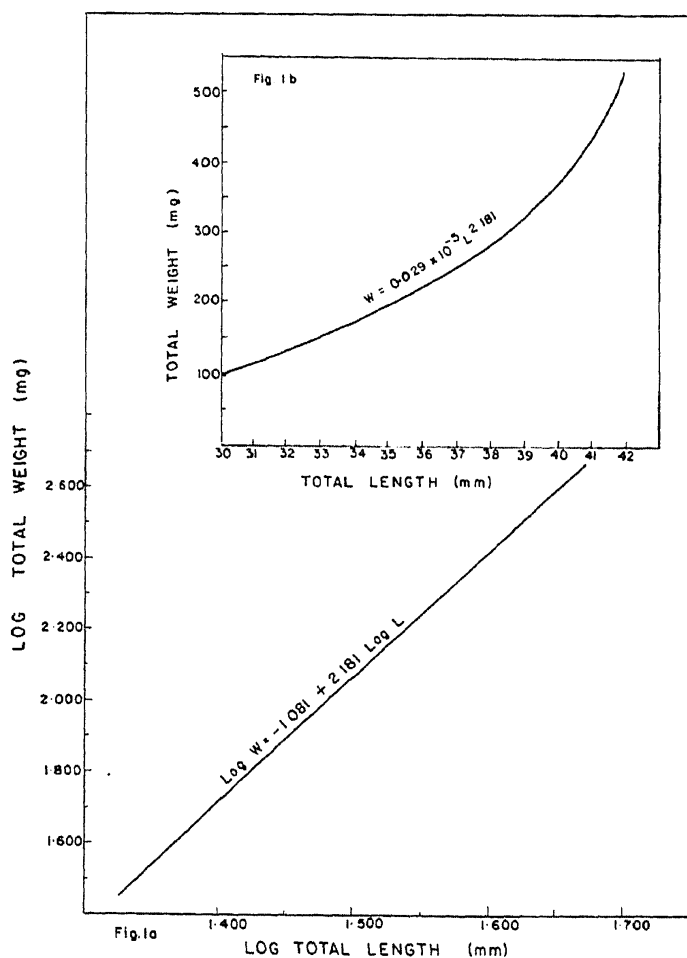
Figure 1. Length-weight relationship in the Antarctic Krill, Euphausia superba . Dana 1850. 1a. Linear regression equation, 1b. Parabolic representation.
