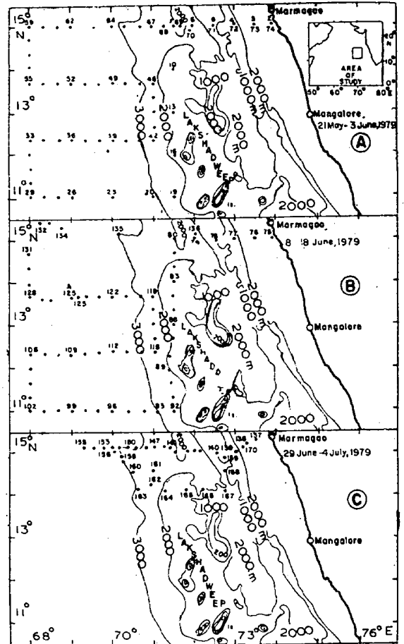
Fig. 1. Bathythermograph station locations in the east central Arabian Sea during MONEX '79 period
