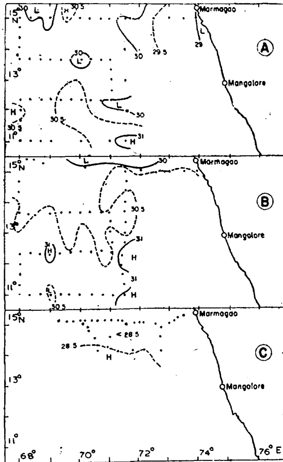
Fig. 4. SST (°C) in the east central Arabian Sea during the three phases
