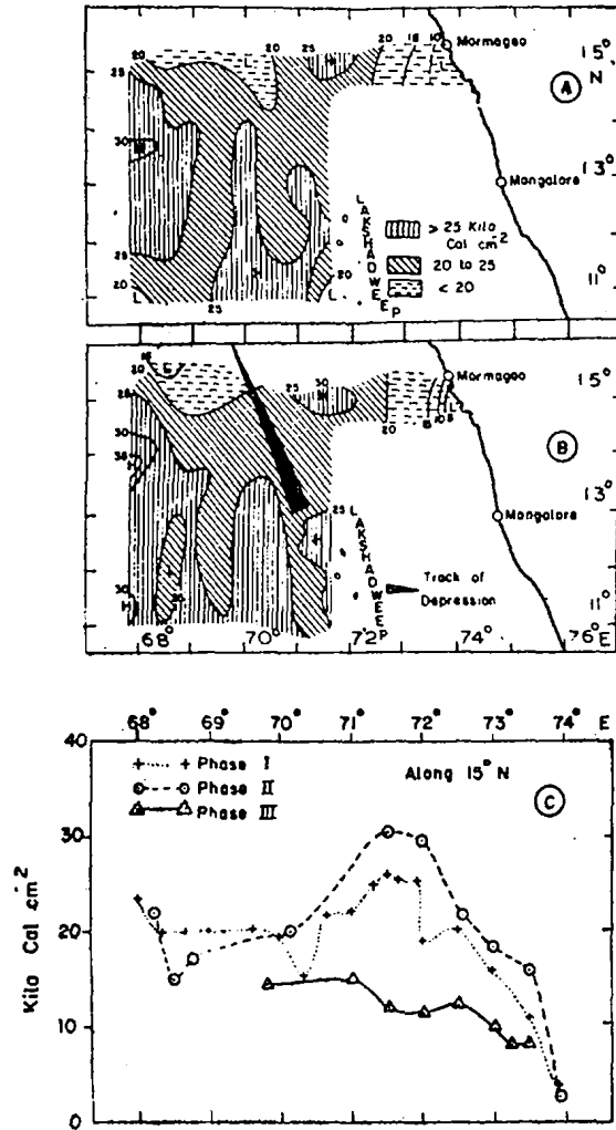
Fig. 7 (A-C), Cyclone heat potential (kilo cal cm -2 ) in the east central Arabian Sea during first phase (A), second phase (B) and along 15°N during three phases (C)
