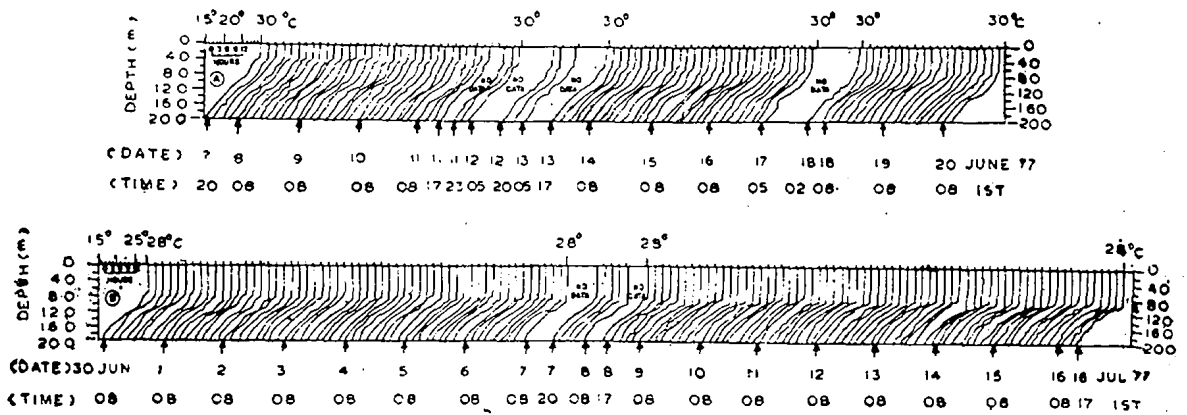
Fig. 8. Time series depth-temperature profiles at RV Shirshov location (12.5°N & 68°E) during first phase (A) and second phase (B) of MONSOON '77 programme
