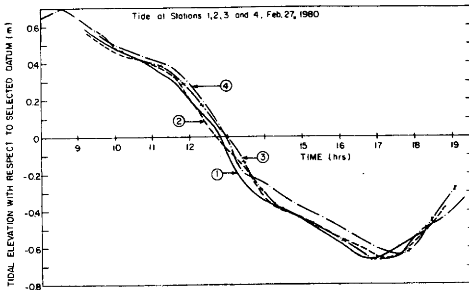
Fig. 5. Tide measurements at stations 1, 2, 3 and 4 on February 27, 1980.
