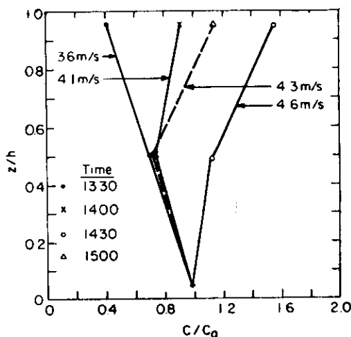
Fig. 11. Normalized suspended sediment concentration, C/C_0 , against relative elevation, z/h , at four wind speeds (measured at 1.5 m elevation above the water surface).
