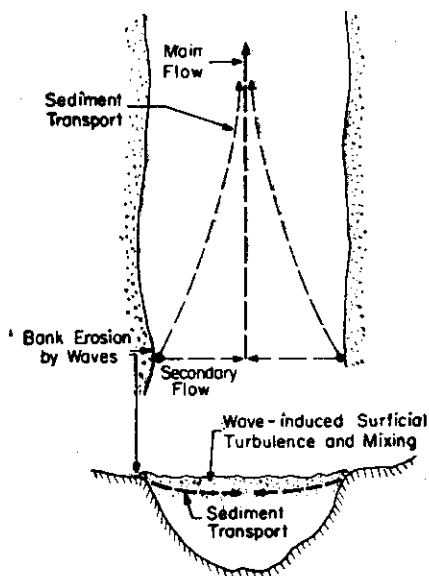
Fig. 10. Transport of bank-derived suspended sediment in the presence of wind-generated waves.
