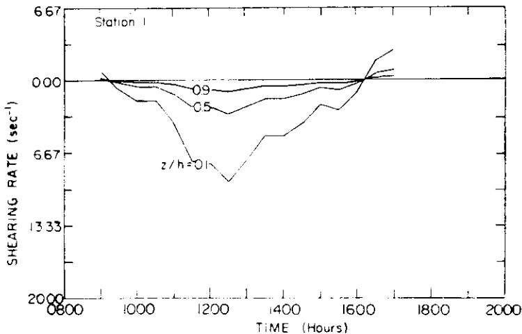
Fig. 7. Shearing rates in the canal at relative elevations z/h = 0.1, 0.5 and 0.9 at station 1.
