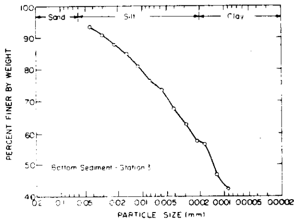
Fig. 4. Grain size distribution of the bottom sediment at station 3, near Cundaim.
