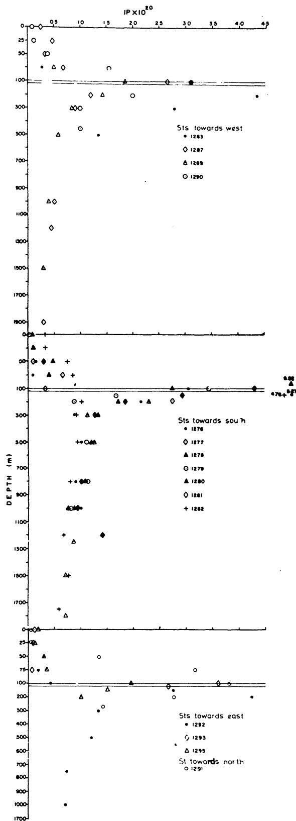
Fig. 2—Depth profile of ionic product of calcium phosphate at stations around the Andaman Island
