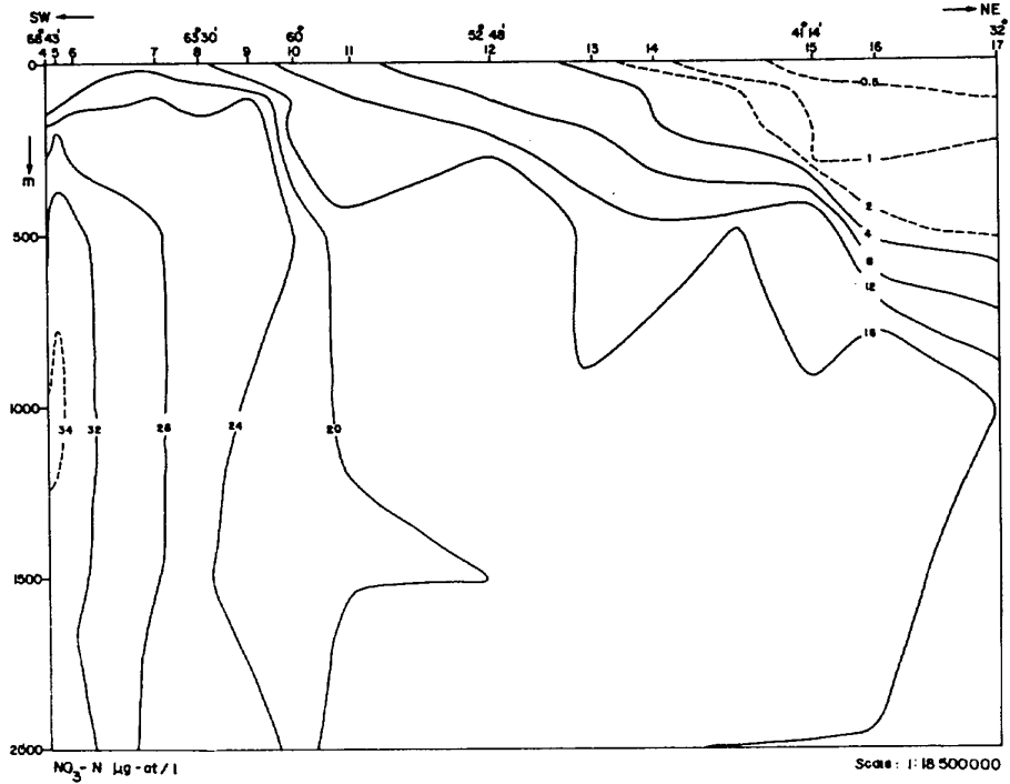
Fig. 4 : Isopleths of nitrate-nitrogen along the section.
