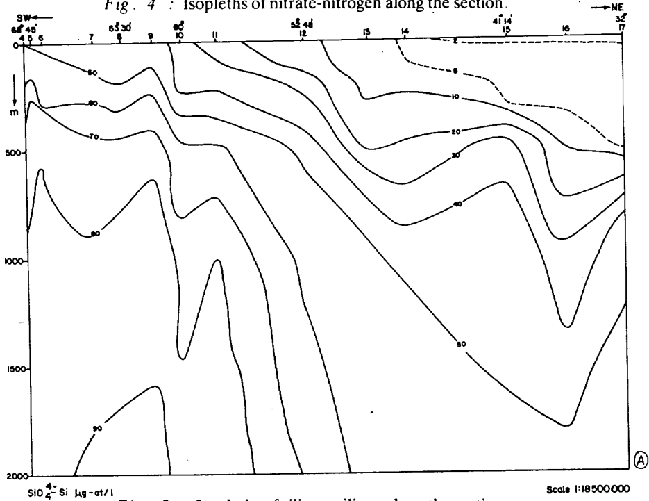
Fig. 5 : Isopleths of silicate-silicon along the section
