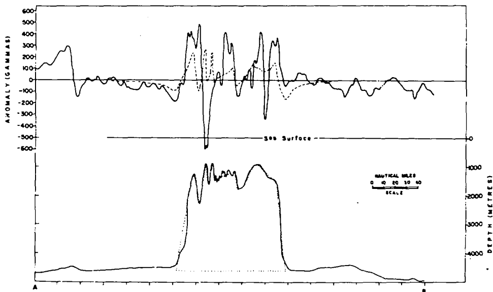
Fig. 3 : A simplified cross section (A to B) of the Indira Mount with its associated magnetic anomalies. Both observed and computed anomalies have been shown in the figure. In the top figure, solid lines show observed magnetic anomalies and broken line, computed anomalies. In the bottom part of the figure, solid line gives the bathymetric profile of the Indira Mount. Dotted line shows the outline of the assumed body (see text).
