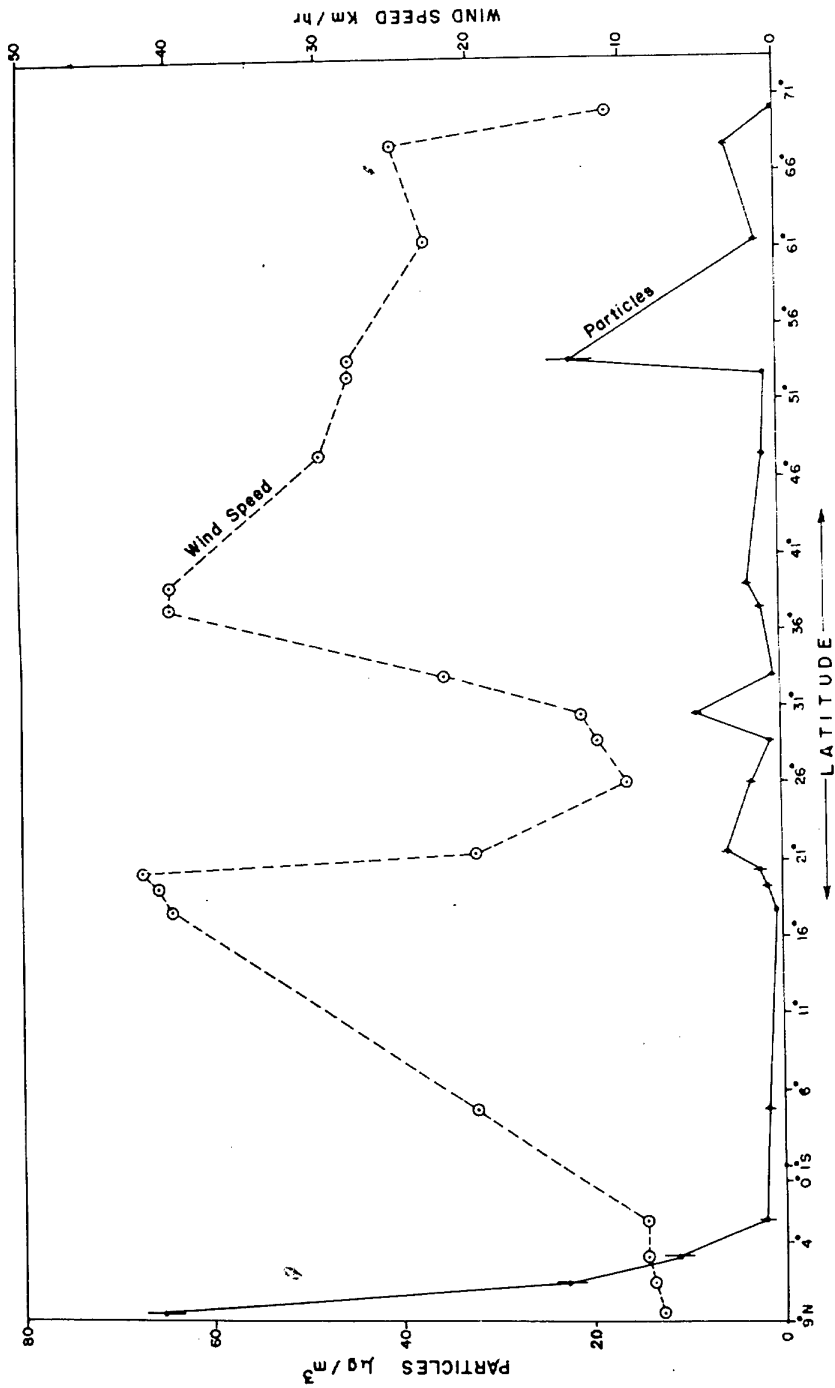
Fig. 2 : Variation of particles and wind speed with latitudes
